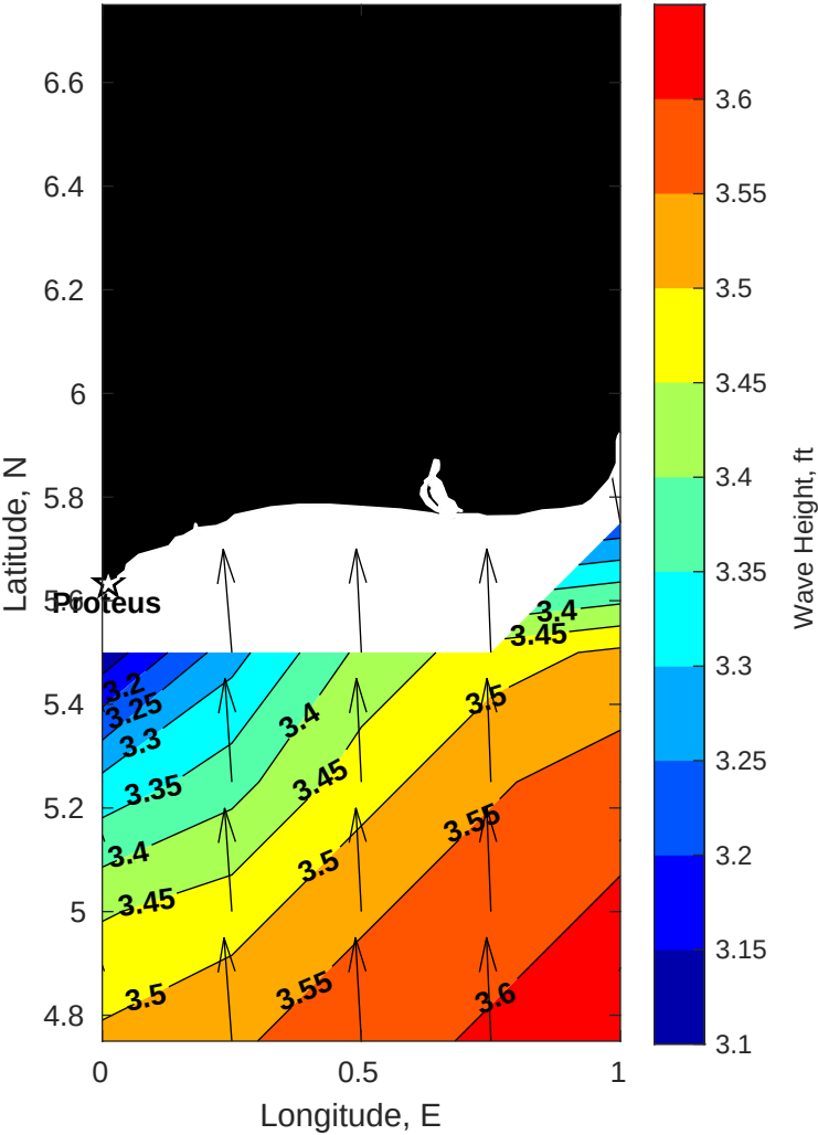
Wave Height (ft) for Proteus at 07-Apr-2025 09:00:00
