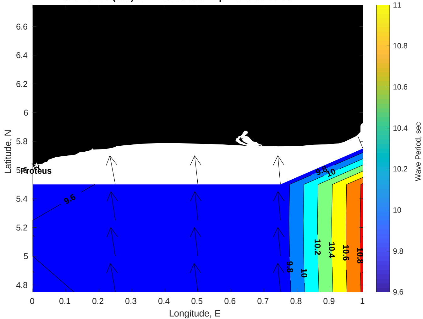
Wave Period (sec) for Proteus at 07-Apr-2025 09:00:00
