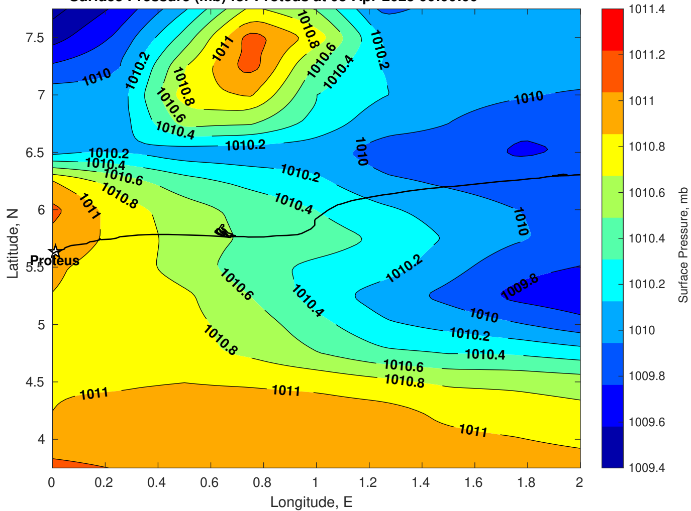
Surface Pressure (mb) for Proteus at 08-Apr-2025 00:00:00
