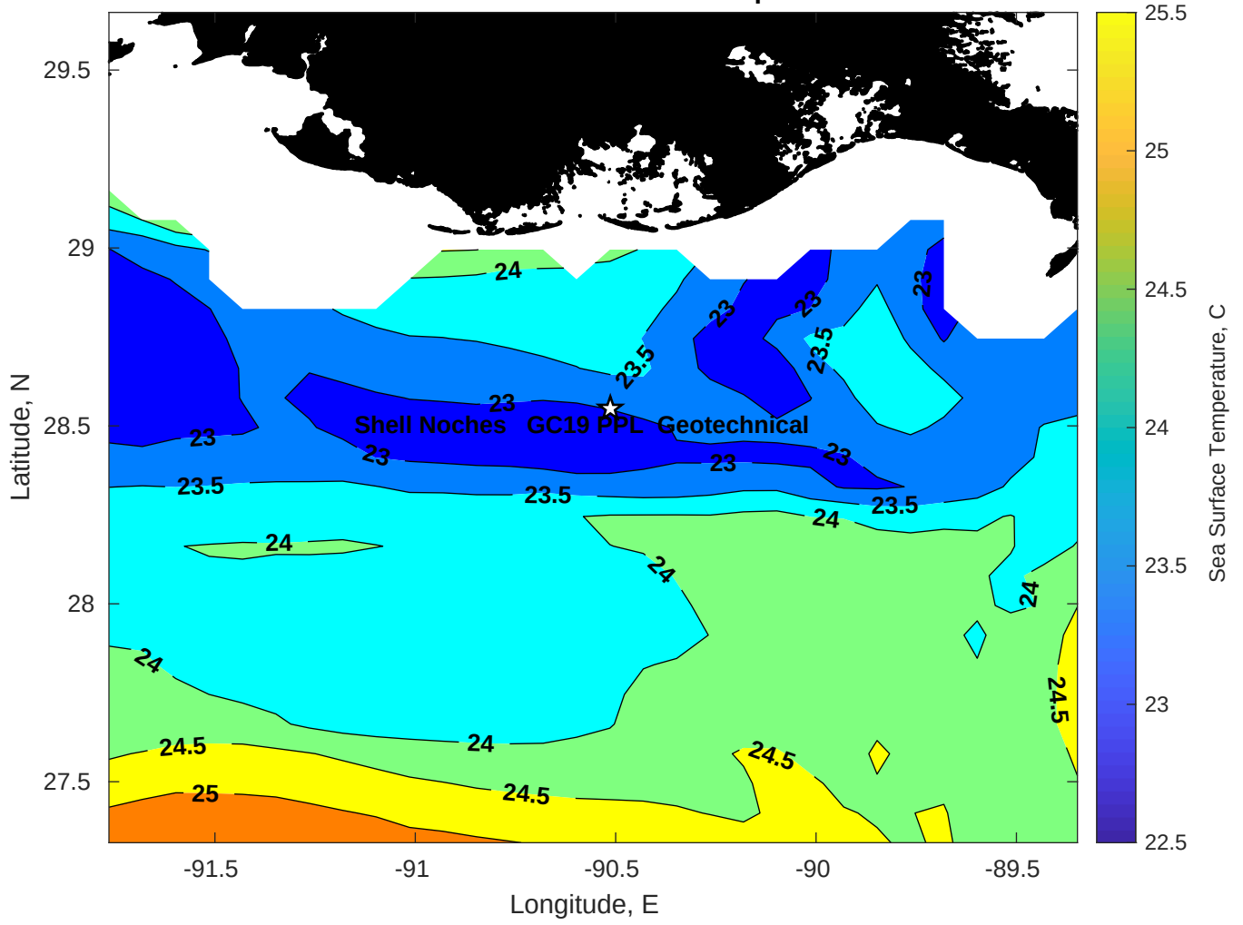
SST for Shell Noches GC19 PPL Geotechnical at 06-Apr-2025 00:00:00
