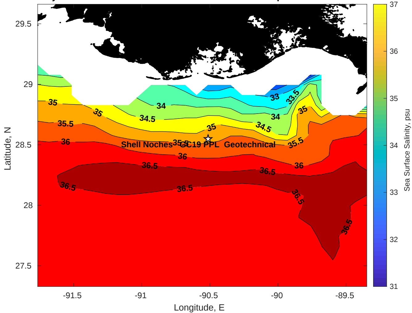
Surface Salinity for Shell Noches GC19 PPL Geotechnical at 06-Apr-2025 00:00:00
