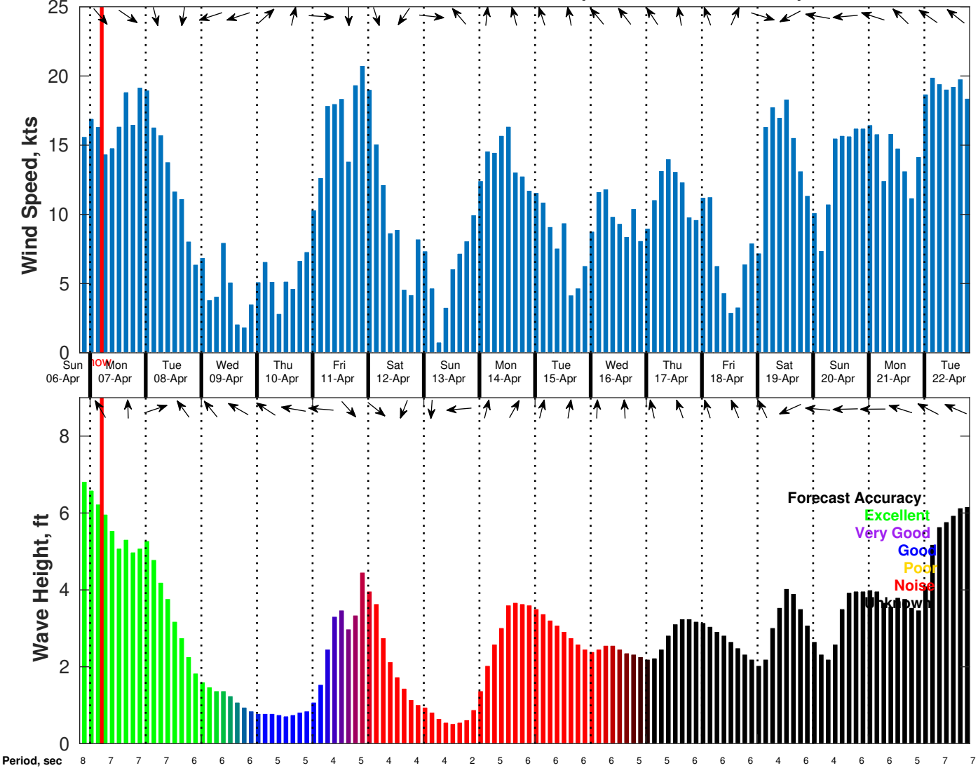
Wind & Wave Forecast for Shell Noches GC19 PPL Geotechnical from 06-Apr-2025 20:00:00 to 22-Apr-2025 20:00:00
