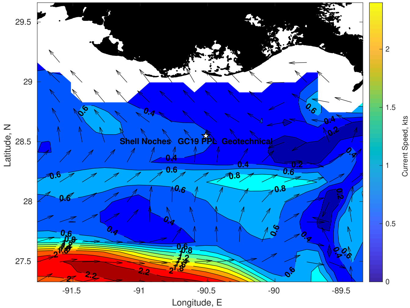
Surface Currents for Shell Noches GC19 PPL Geotechnical at 06-Apr-2025 00:00:00
