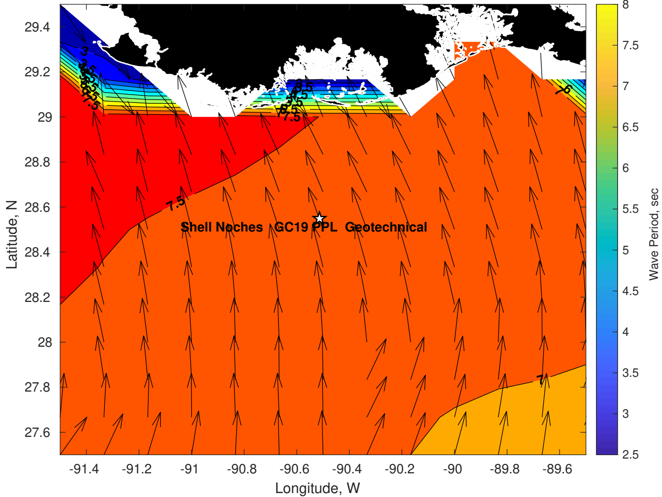
Wave Period (sec) for Shell Noches GC19 PPL Geotechnical at 07-Apr-2025 09:00:00
