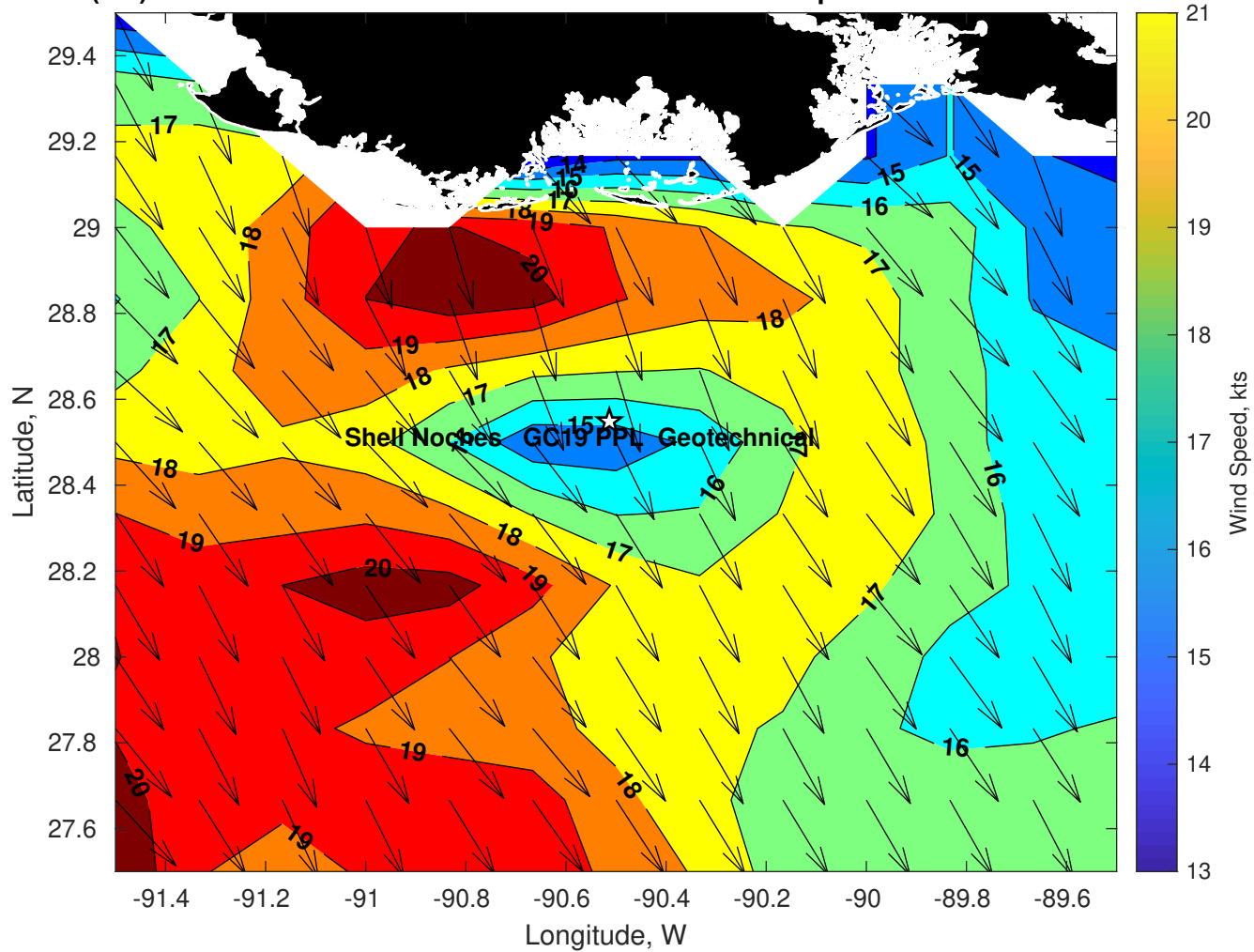
Winds (kts) for Shell Noches GC19 PPL Geotechnical at 07-Apr-2025 09:00:00
