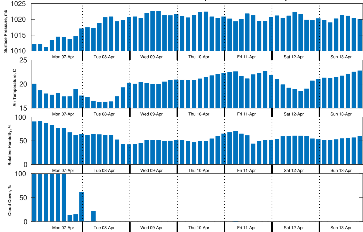
Met Forecast for Shell Noches GC19 PPL Geotechnical from 07-Apr-2025 00:00:00 to 14-Apr-2025 00:00:00
