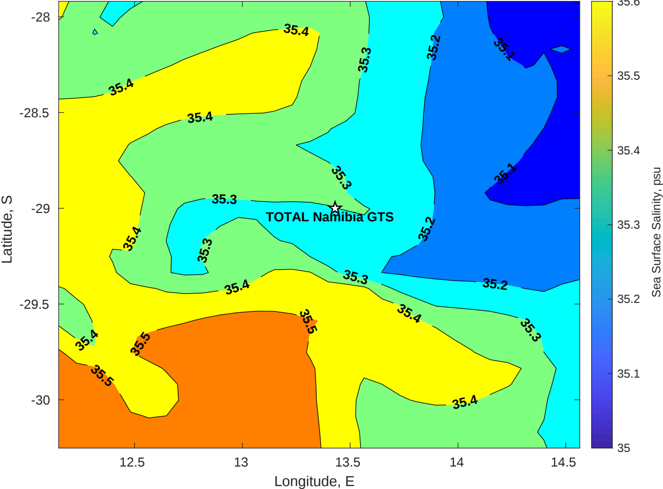
Surface Salinity for TOTAL Namibia GTS at 06-Apr-2025 00:00:00
