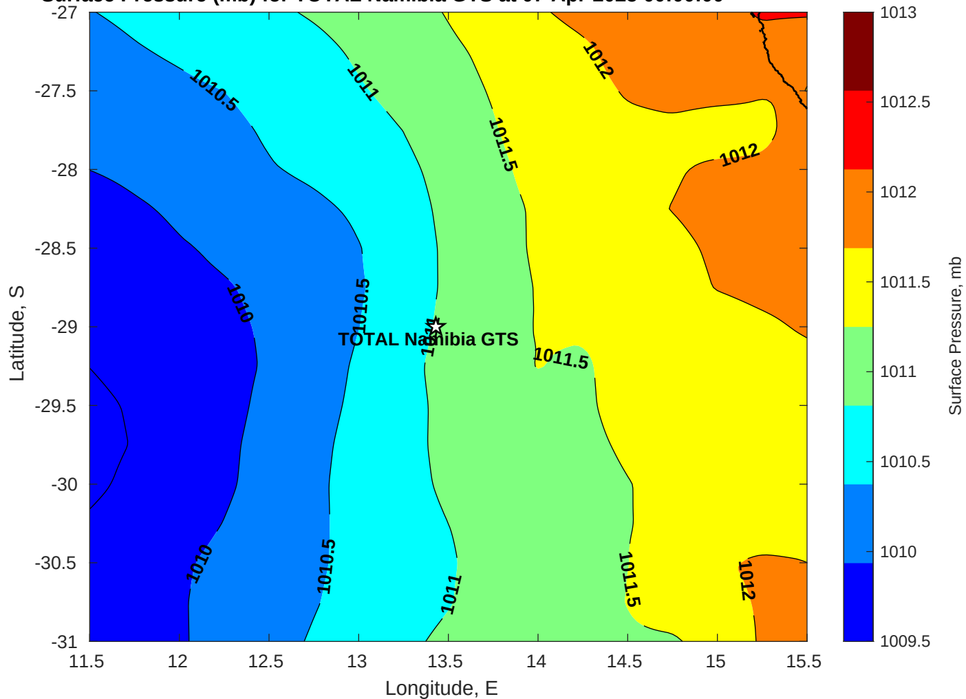
Surface Pressure (mb) for TOTAL Namibia GTS at 07-Apr-2025 00:00:00
