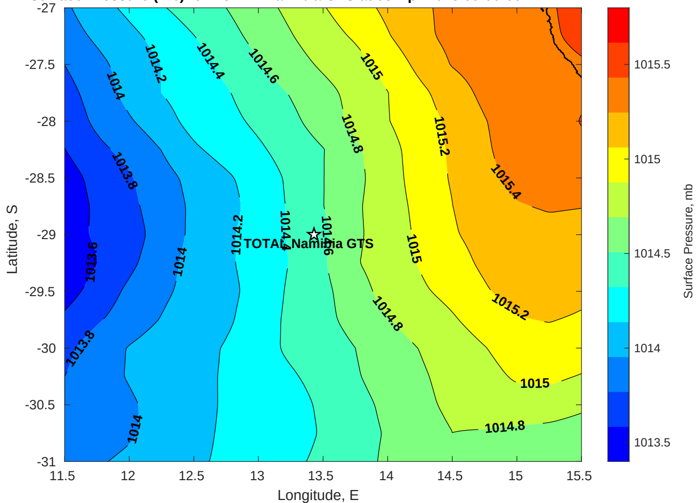
Surface Pressure (mb) for TOTAL Namibia GTS at 08-Apr-2025 00:00:00
