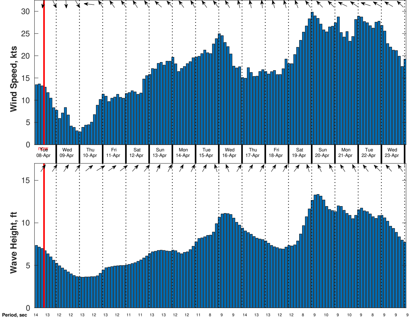
Wind & Wave Forecast for TOTAL Namibia GTS from 07-Apr-2025 02:00:00 to 23-Apr-2025 02:00:00
