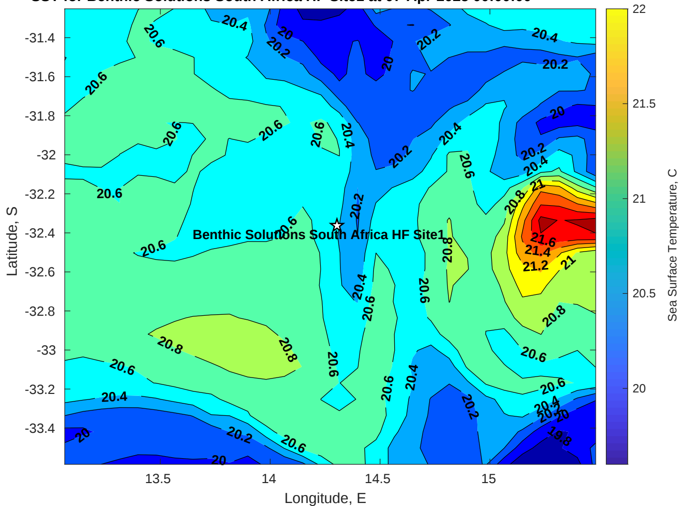
SST for Benthic Solutions South Africa HF Site1 at 07-Apr-2025 00:00:00
