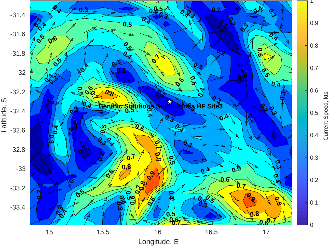
Surface Currents for Benthic Solutions South Africa HF Site3 at 07-Apr-2025 00:00:00
