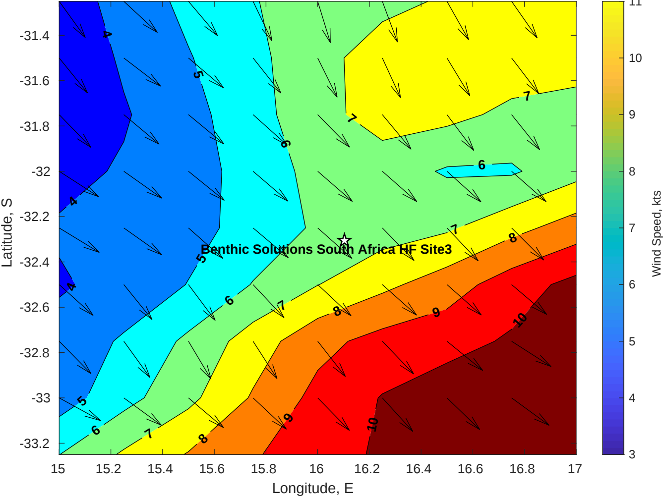
Winds (kts) for Benthic Solutions South Africa HF Site3 at 08-Apr-2025 09:00:00
