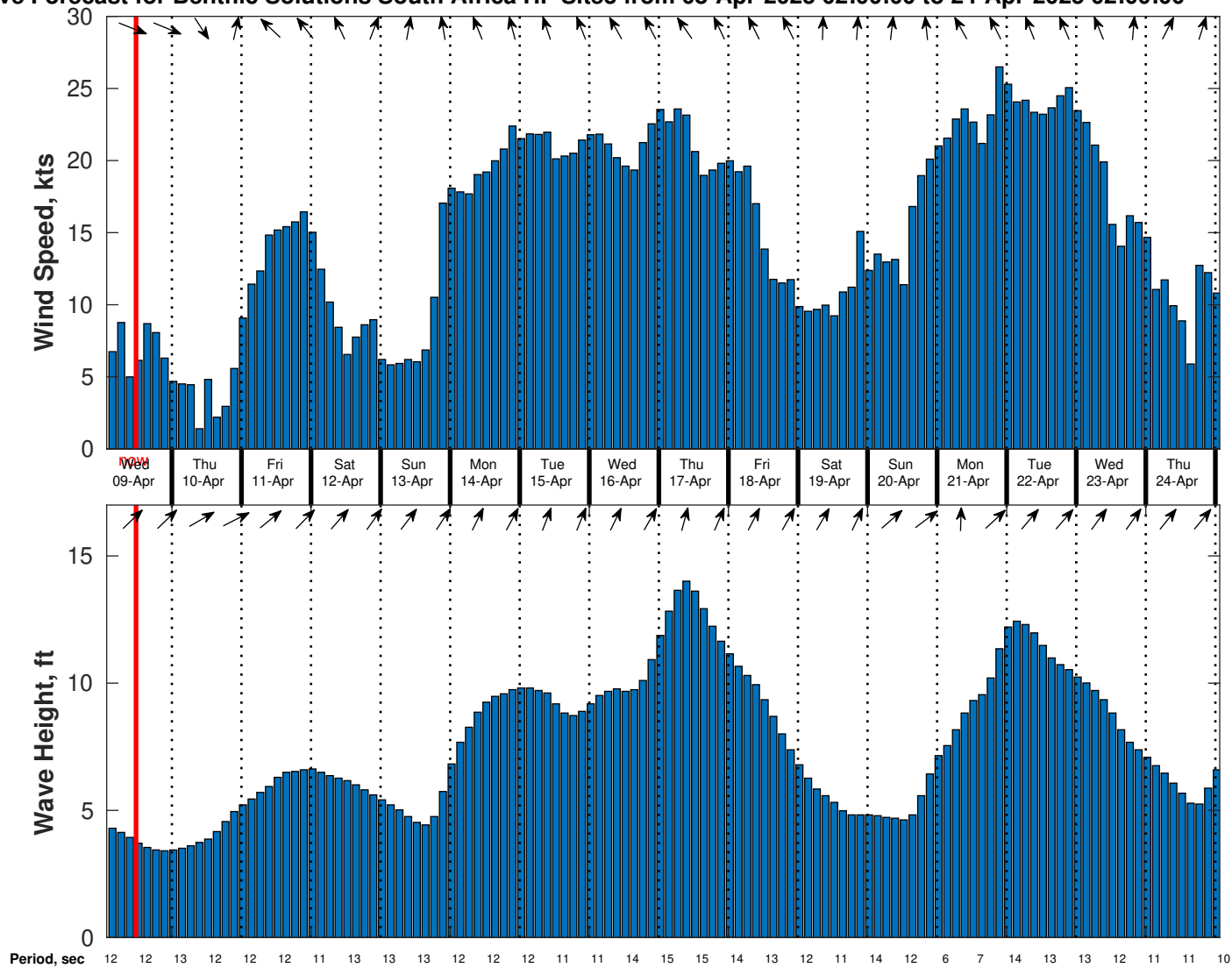
Wind & Wave Forecast for Benthic Solutions South Africa HF Site3 from 08-Apr-2025 02:00:00 to 24-Apr-2025 02:00:00
