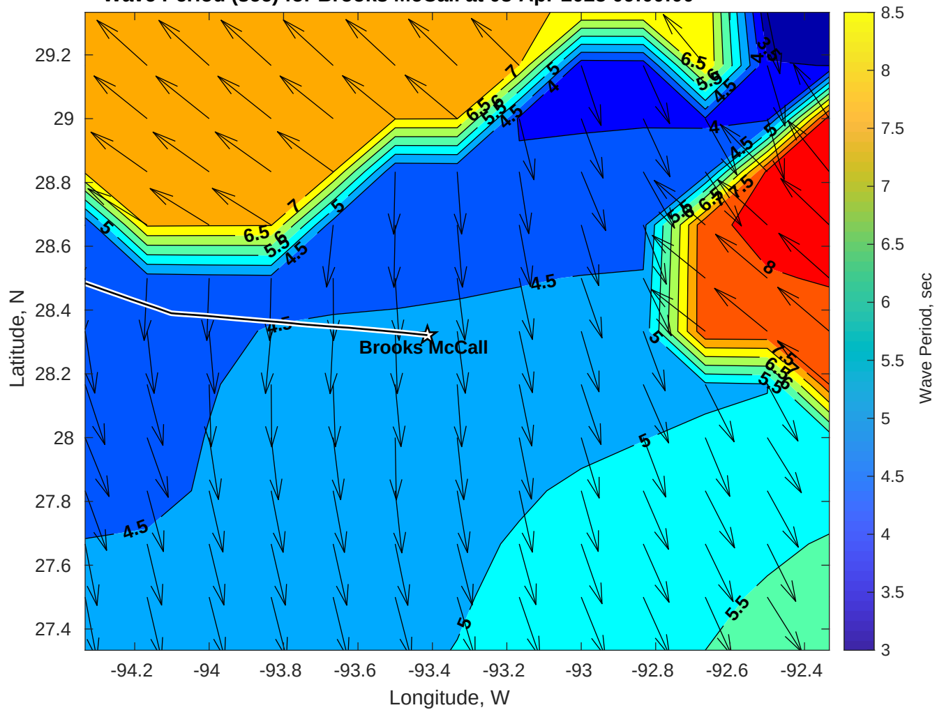
Wave Period (sec) for Brooks McCall at 08-Apr-2025 09:00:00
