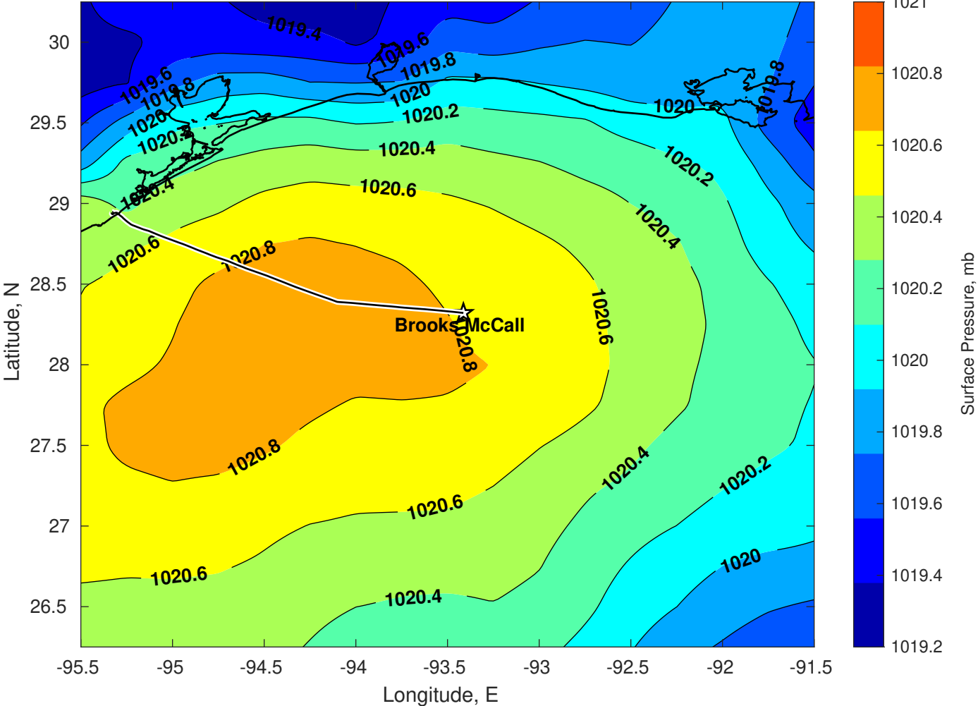
Surface Pressure (mb) for Brooks McCall at 09-Apr-2025 00:00:00
