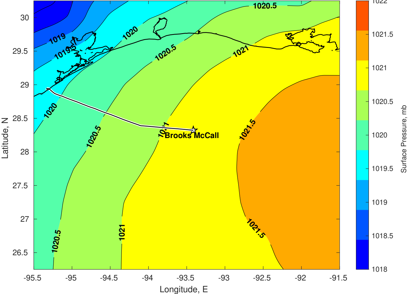
Surface Pressure (mb) for Brooks McCall at 10-Apr-2025 00:00:00
