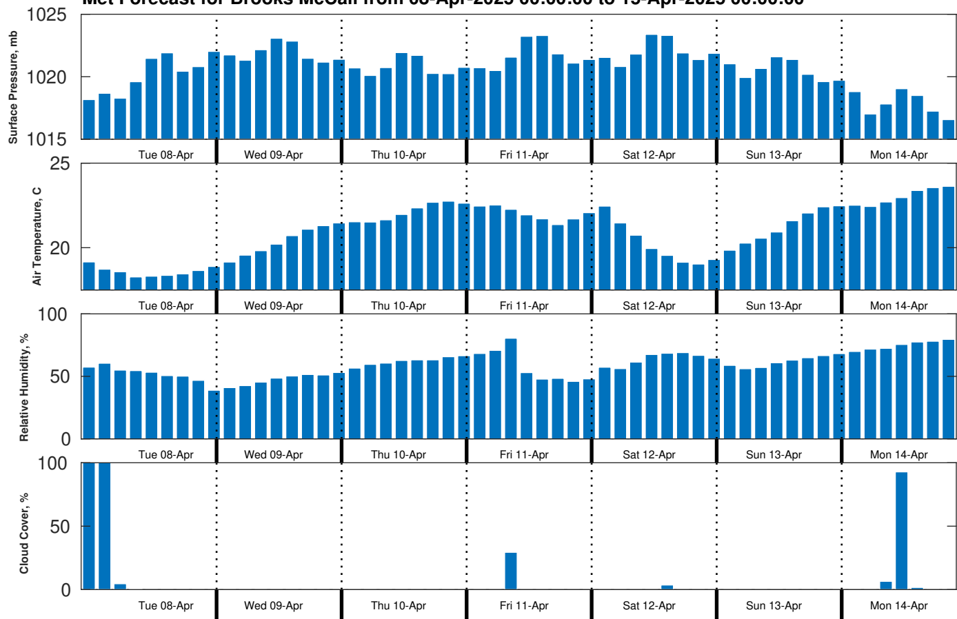
Met Forecast for Brooks McCall from 08-Apr-2025 00:00:00 to 15-Apr-2025 00:00:00
