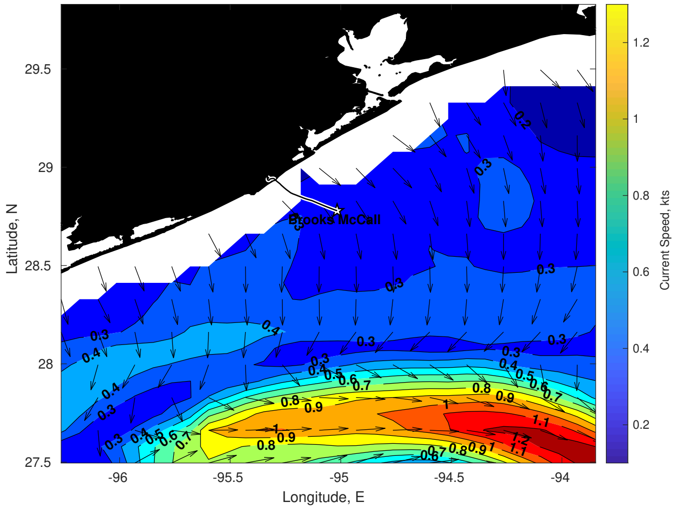
Surface Currents for Brooks McCall at 07-Apr-2025 00:00:00
