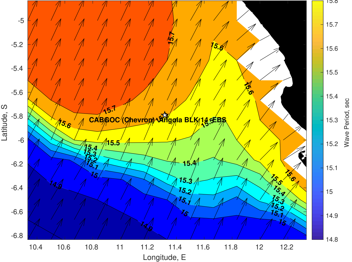
Wave Period (sec) for CABGOC (Chevron) Angola BLK 14 EBS at 08-Apr-2025 09:00:00
