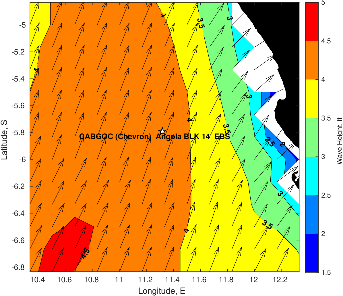
Wave Height (ft) for CABGOC (Chevron) Angola BLK 14 EBS at 08-Apr-2025 09:00:00
