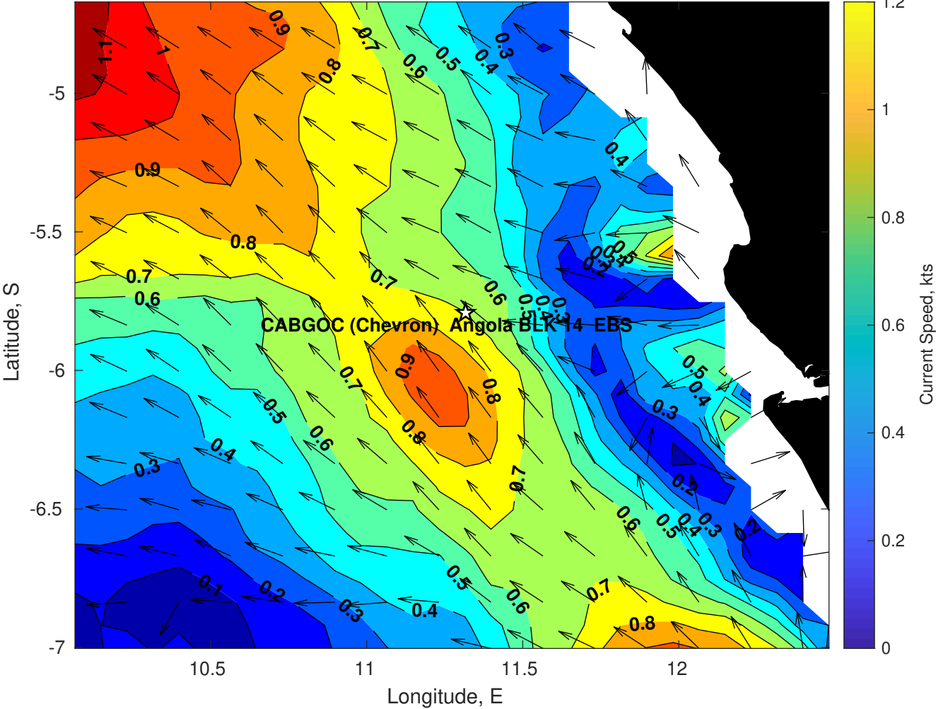
Surface Currents for CABGOC (Chevron) Angola BLK 14 EBS at 07-Apr-2025 00:00:00
