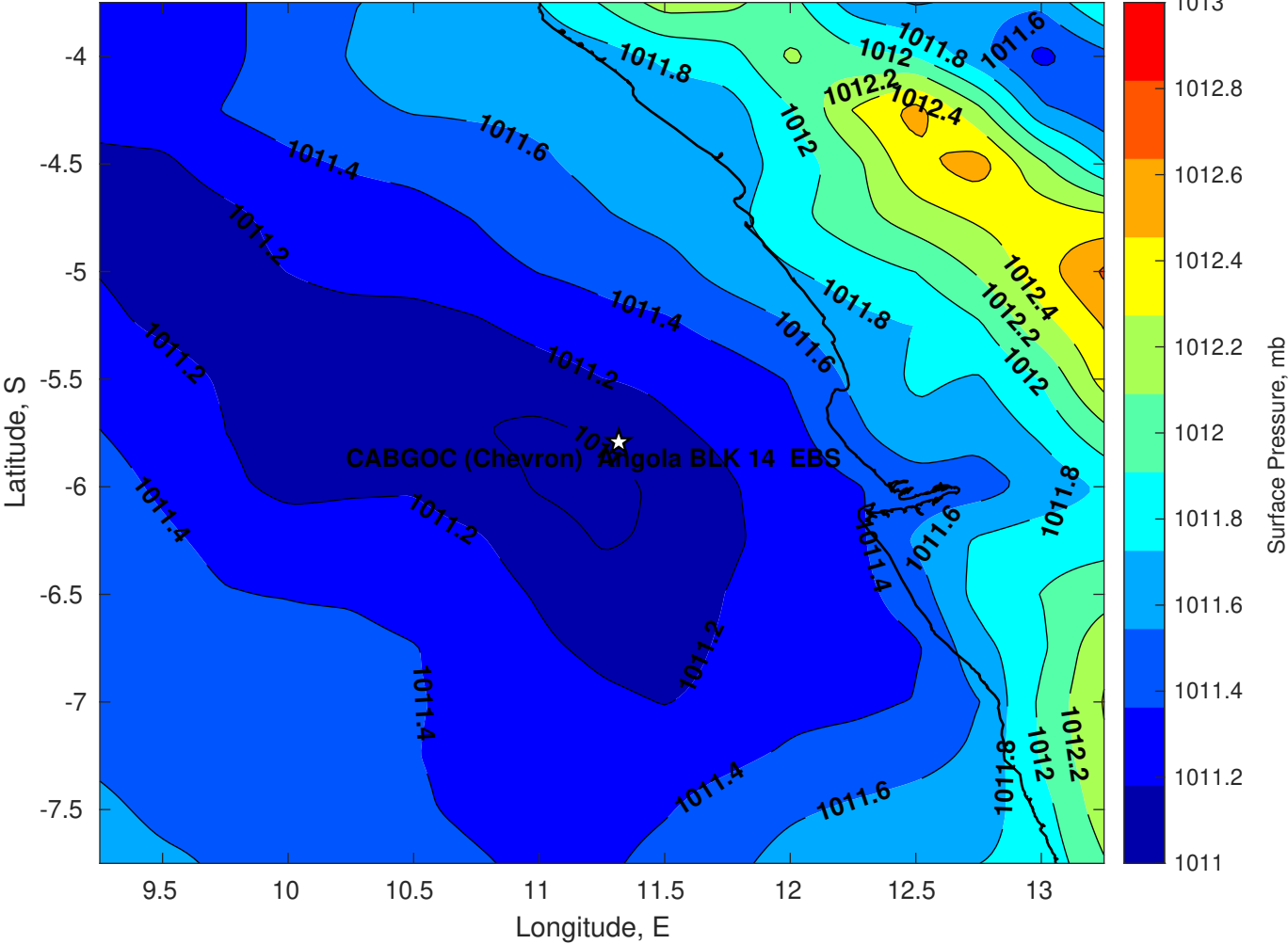
Surface Pressure (mb) for CABGOC (Chevron) Angola BLK 14 EBS at 08-Apr-2025 00:00:00
