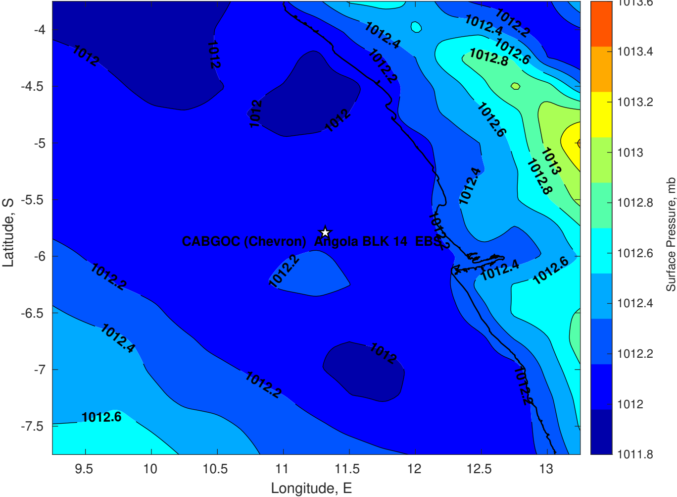
Surface Pressure (mb) for CABGOC (Chevron) Angola BLK 14 EBS at 09-Apr-2025 00:00:00
