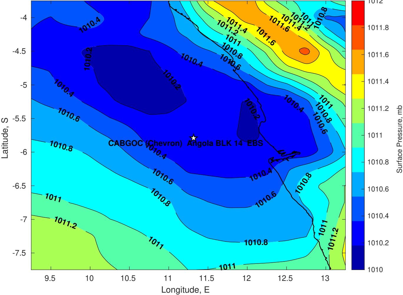
Surface Pressure (mb) for CABGOC (Chevron) Angola BLK 14 EBS at 10-Apr-2025 00:00:00
