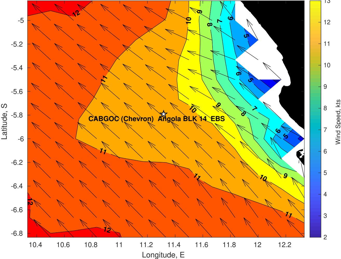
Winds (kts) for CABGOC (Chevron) Angola BLK 14 EBS at 08-Apr-2025 09:00:00
