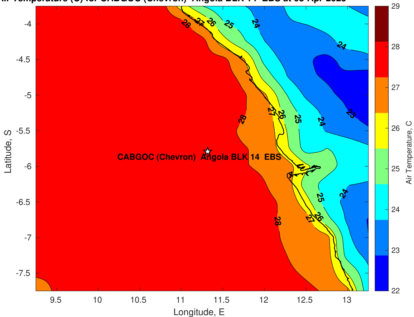
Air Temperature (C) for CABGOC (Chevron) Angola BLK 14 EBS at 08-Apr-2025
