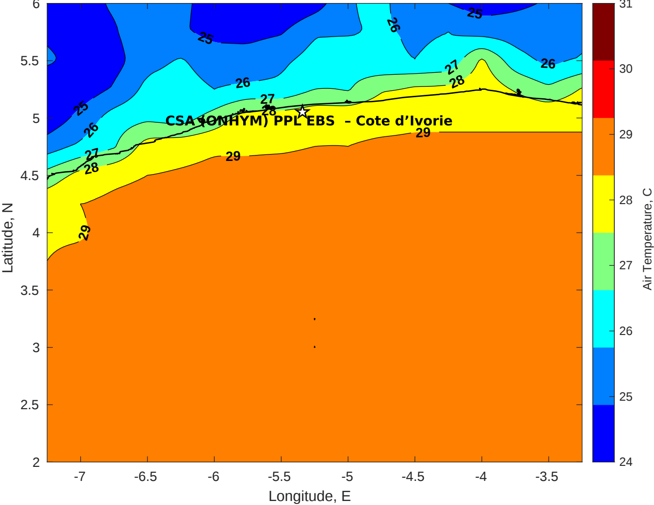
Air Temperature (C) for CSA (ONHYM) PPL EBS - Cote d'Ivoire at 08-Apr-2025
