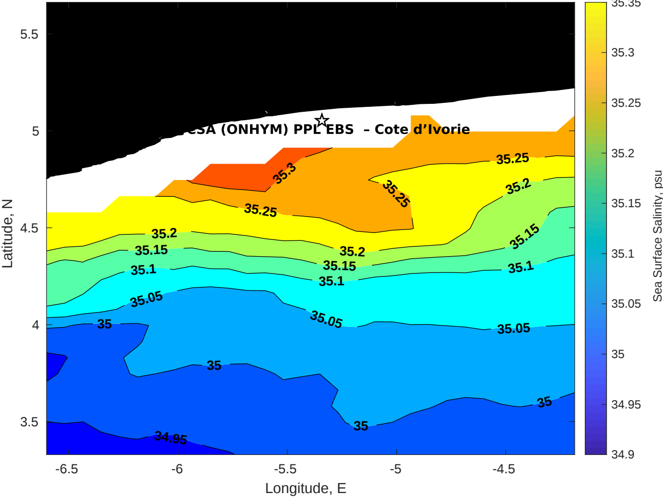
Surface Salinity for CSA (ONHYM) PPL EBS - Cote d'Ivoire at 07-Apr-2025 00:00:00
