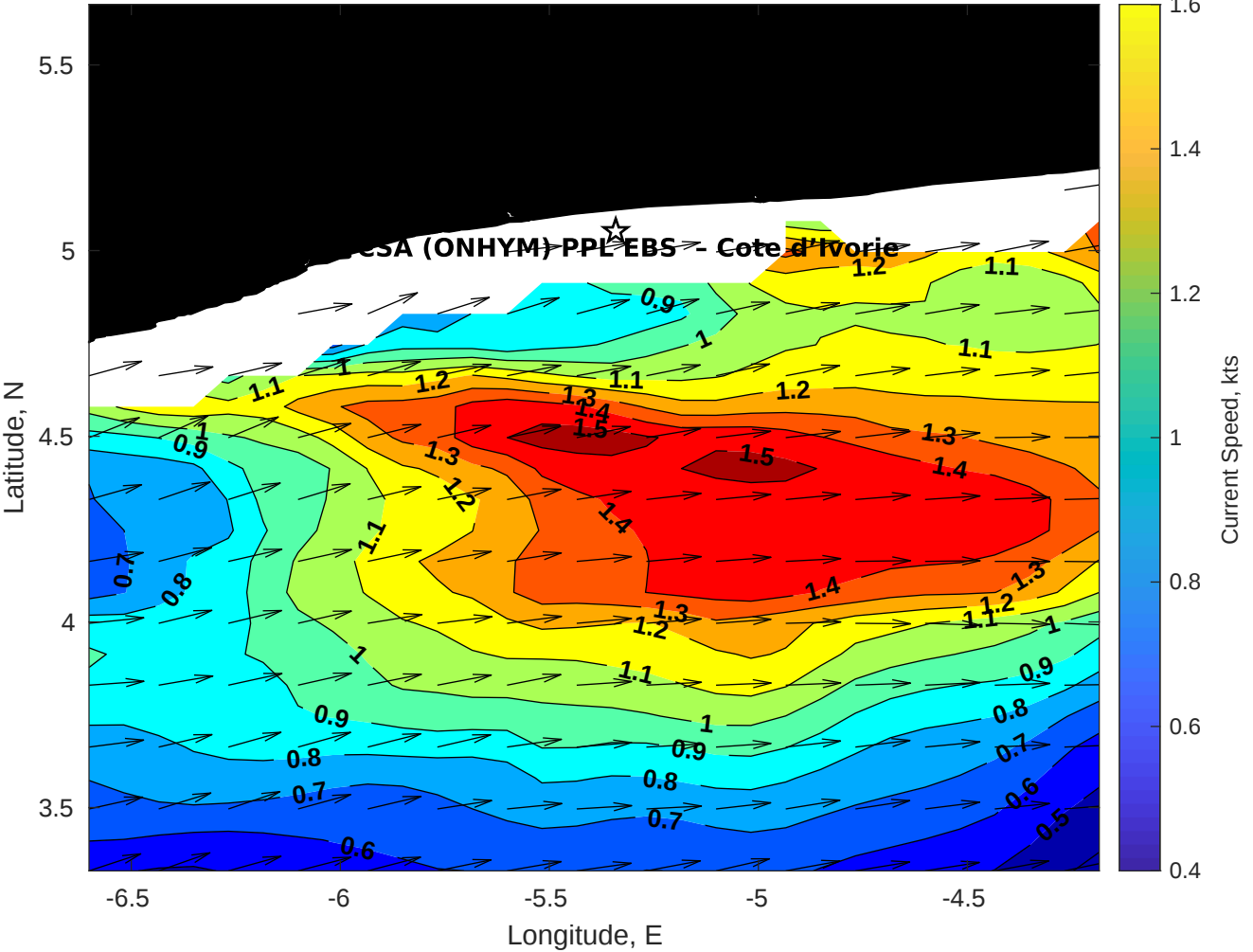
Surface Currents for CSA (ONHYM) PPL EBS - Cote d'Ivoire at 07-Apr-2025 00:00:00
