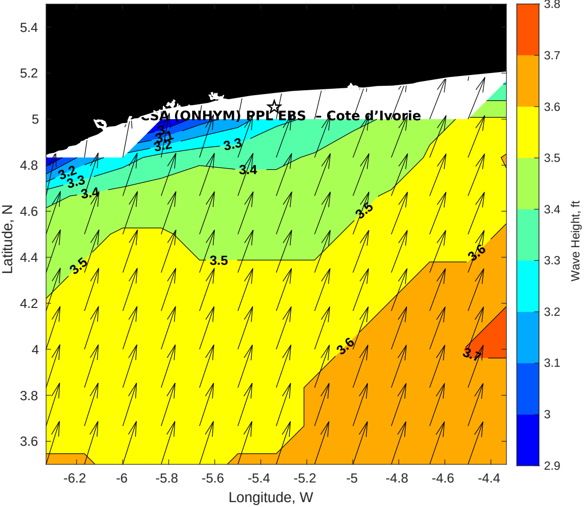
Wave Height (ft) for CSA (ONHYM) PPL EBS - Cote d'Ivoire at 08-Apr-2025 09:00:00
