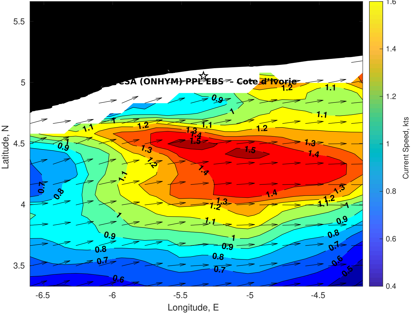
Surface Currents for CSA (ONHYM) PPL EBS - Cote d'Ivoire at 07-Apr-2025 00:00:00
