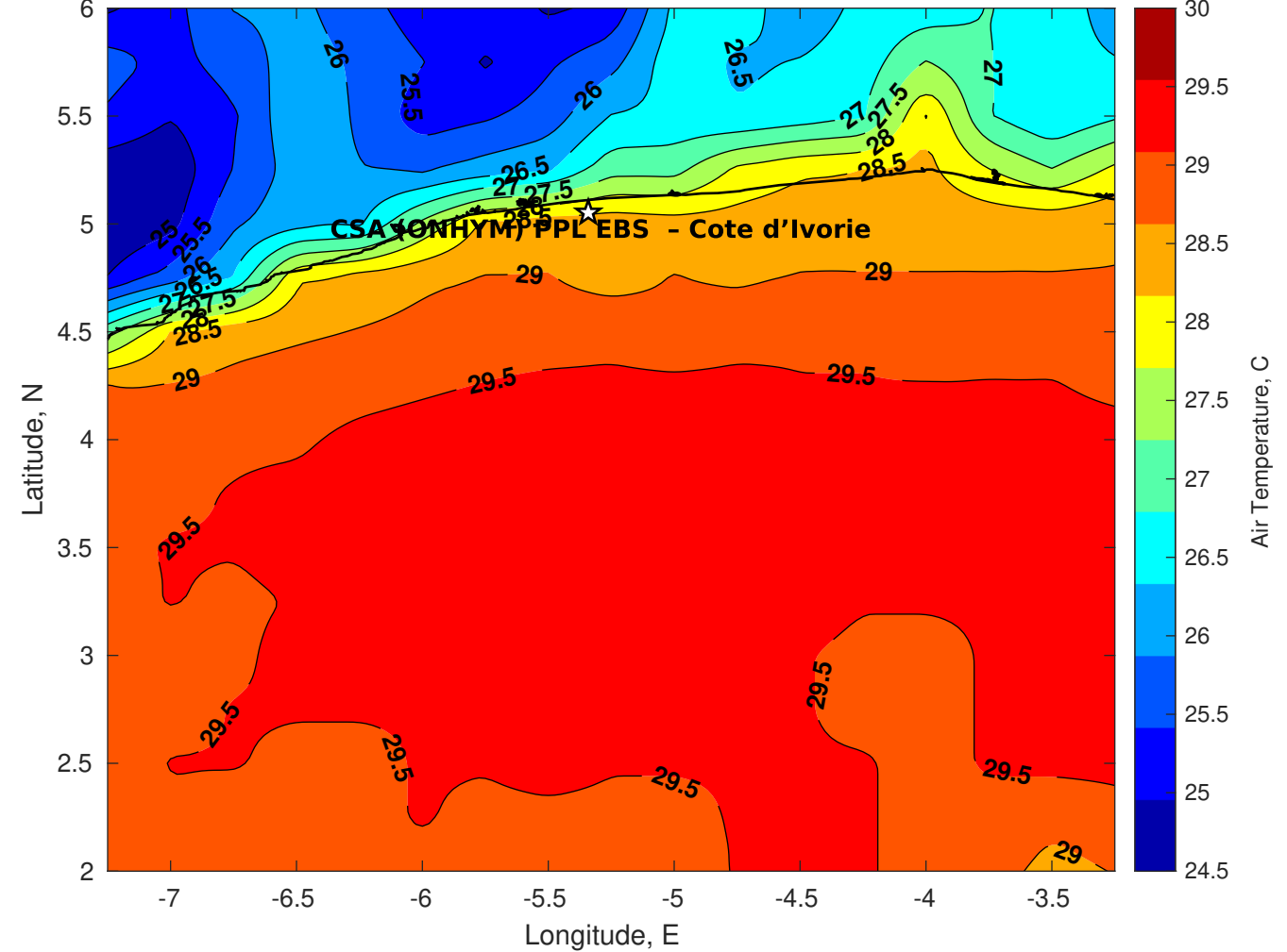
Air Temperature (C) for CSA (ONHYM) PPL EBS - Cote d'Ivoire at 08-Apr-2025
