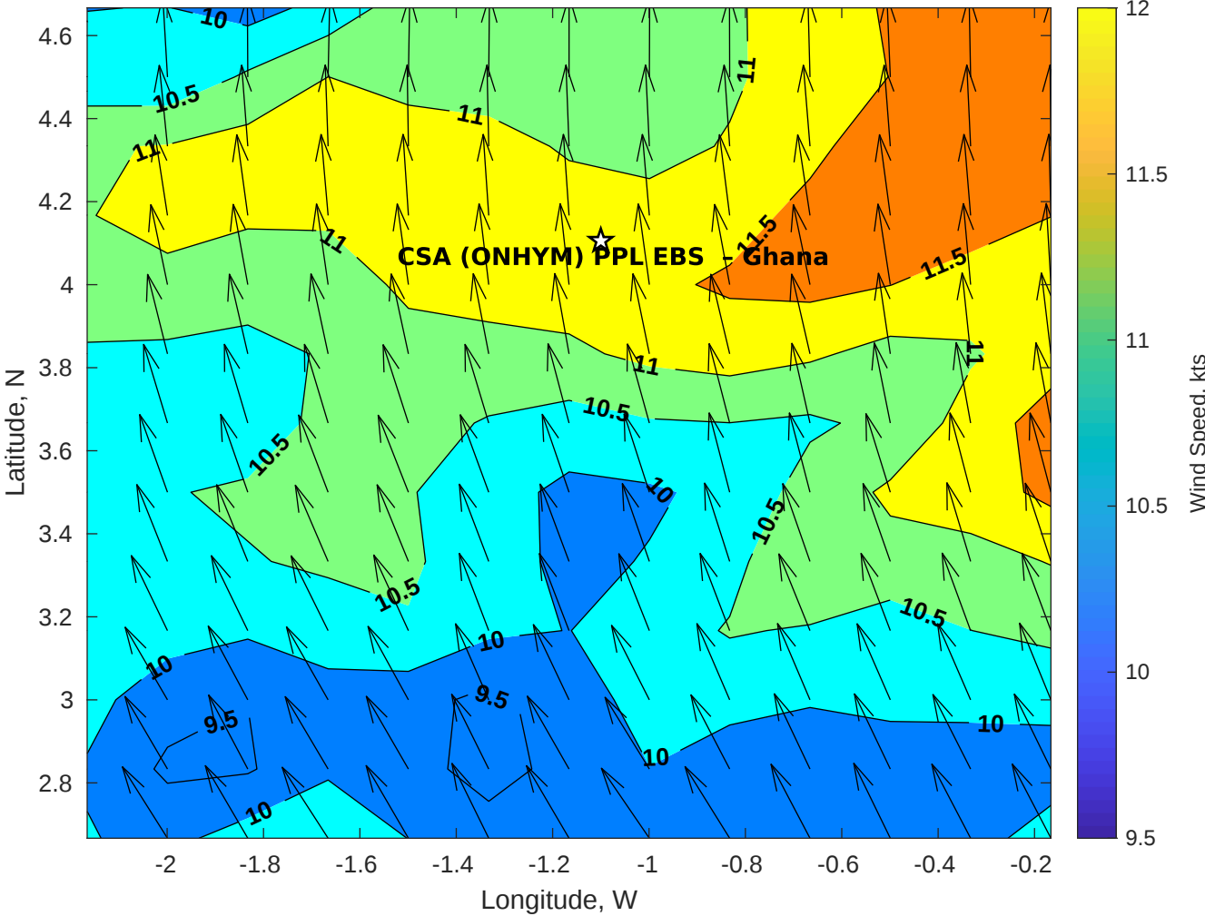
Winds (kts) for CSA (ONHYM) PPL EBS - Ghana at 08-Apr-2025 09:00:00
