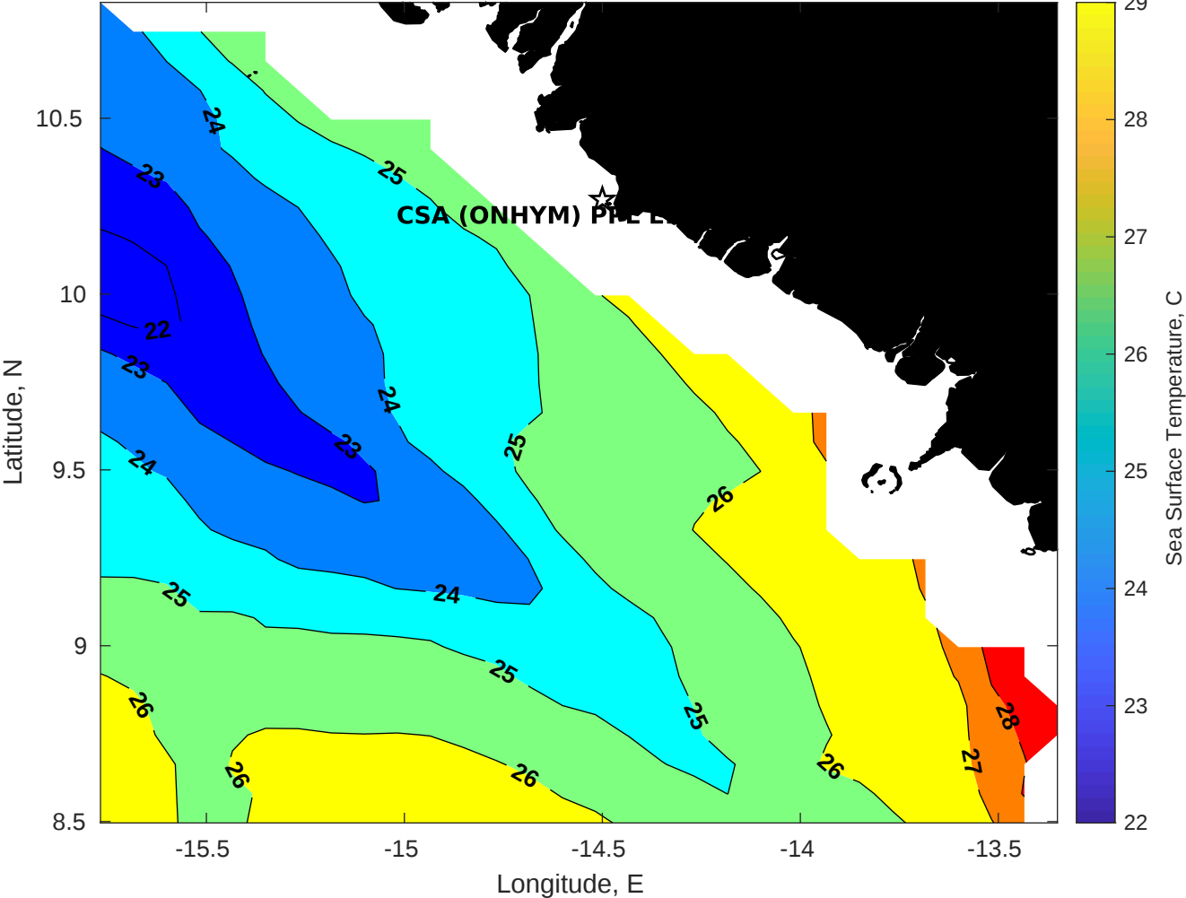
SST for CSA (ONHYM) PPL EBS - Guinea at 07-Apr-2025 00:00:00
