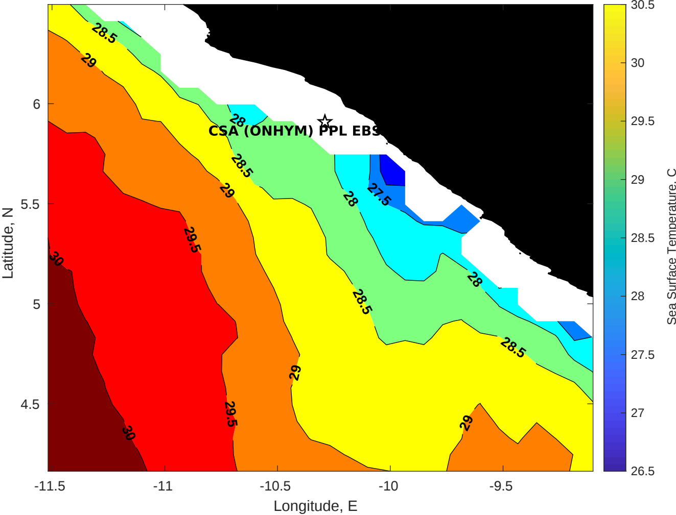
SST for CSA (ONHYM) PPL EBS - Liberia at 07-Apr-2025 00:00:00
