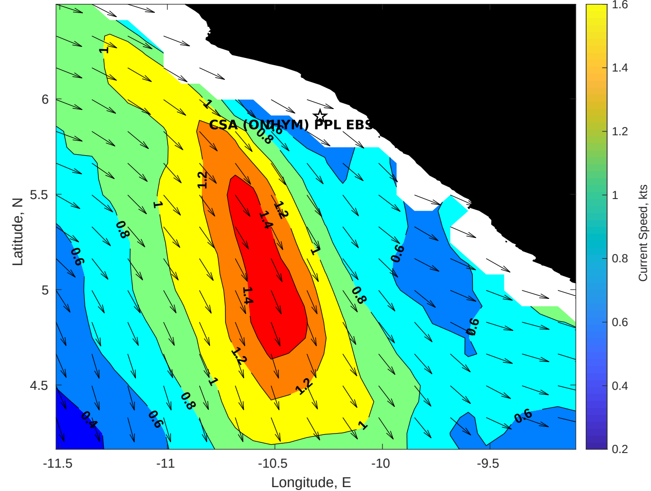
Surface Currents for CSA (ONHYM) PPL EBS - Liberia at 07-Apr-2025 00:00:00
