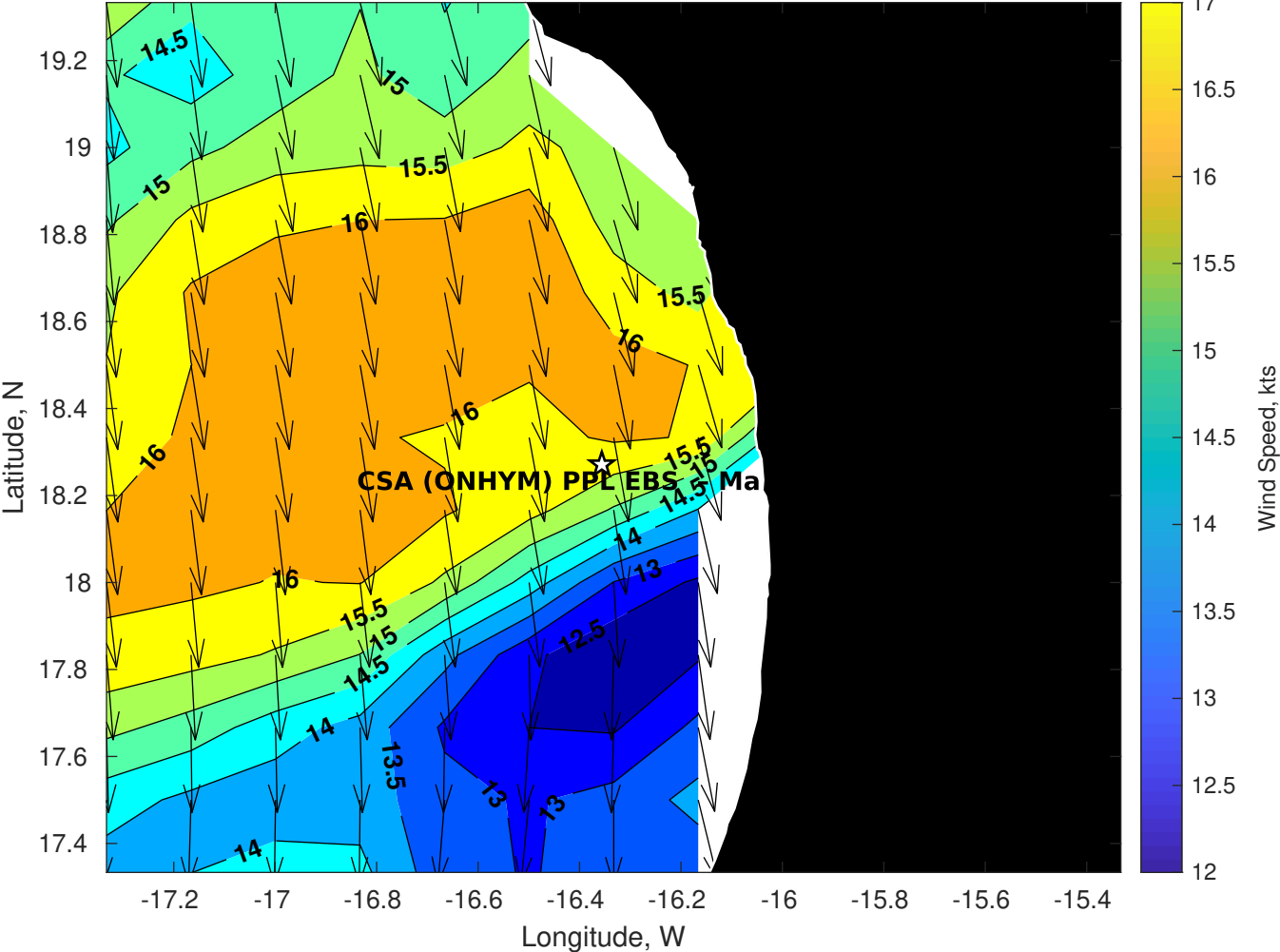
Winds (kts) for CSA (ONHYM) PPL EBS - Mauritania at 08-Apr-2025 09:00:00
