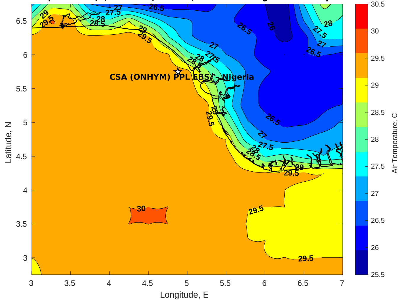
Air Temperature (C) for CSA (ONHYM) PPL EBS - Nigeria at 08-Apr-2025
