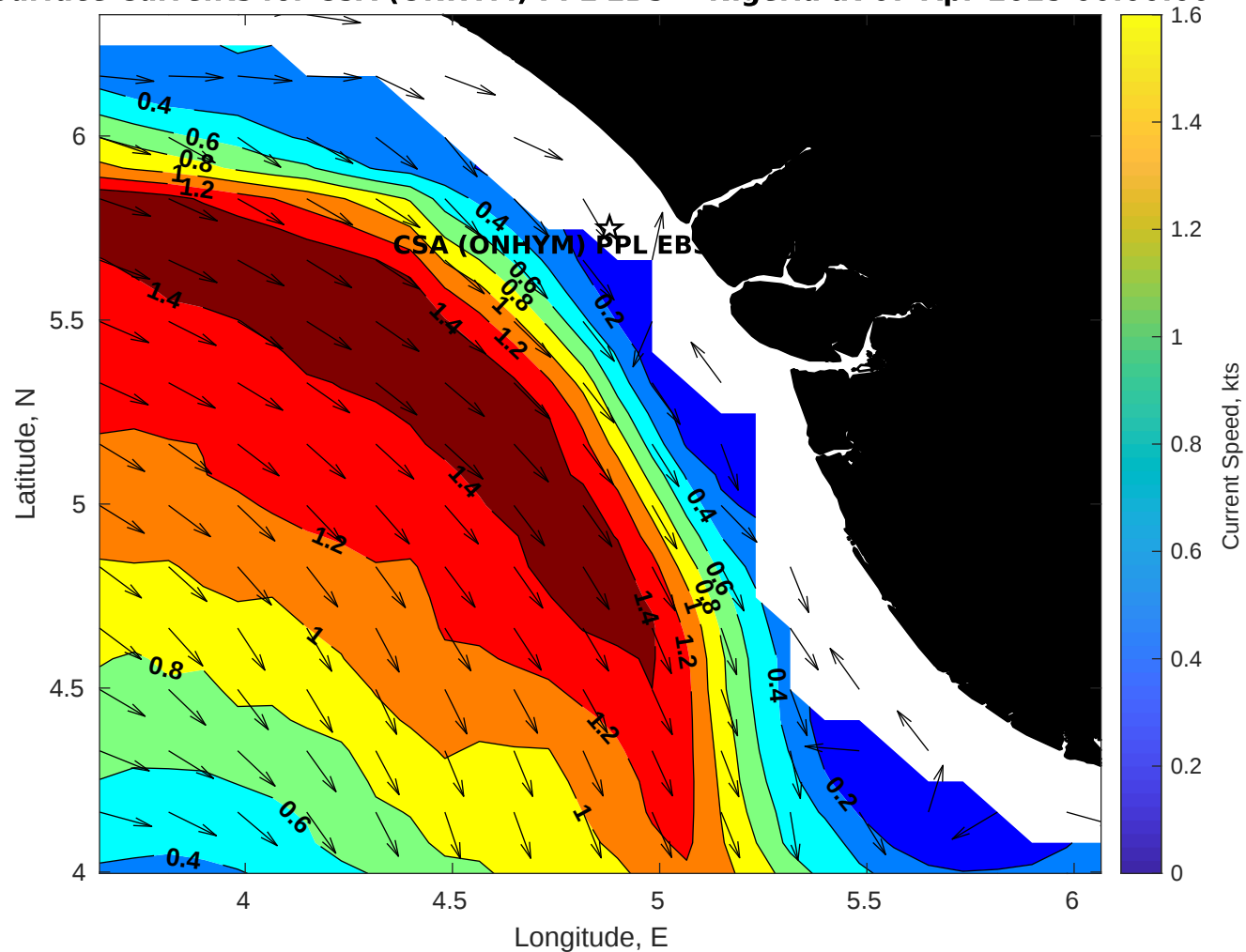
Surface Currents for CSA (ONHYM) PPL EBS - Nigeria at 07-Apr-2025 00:00:00
