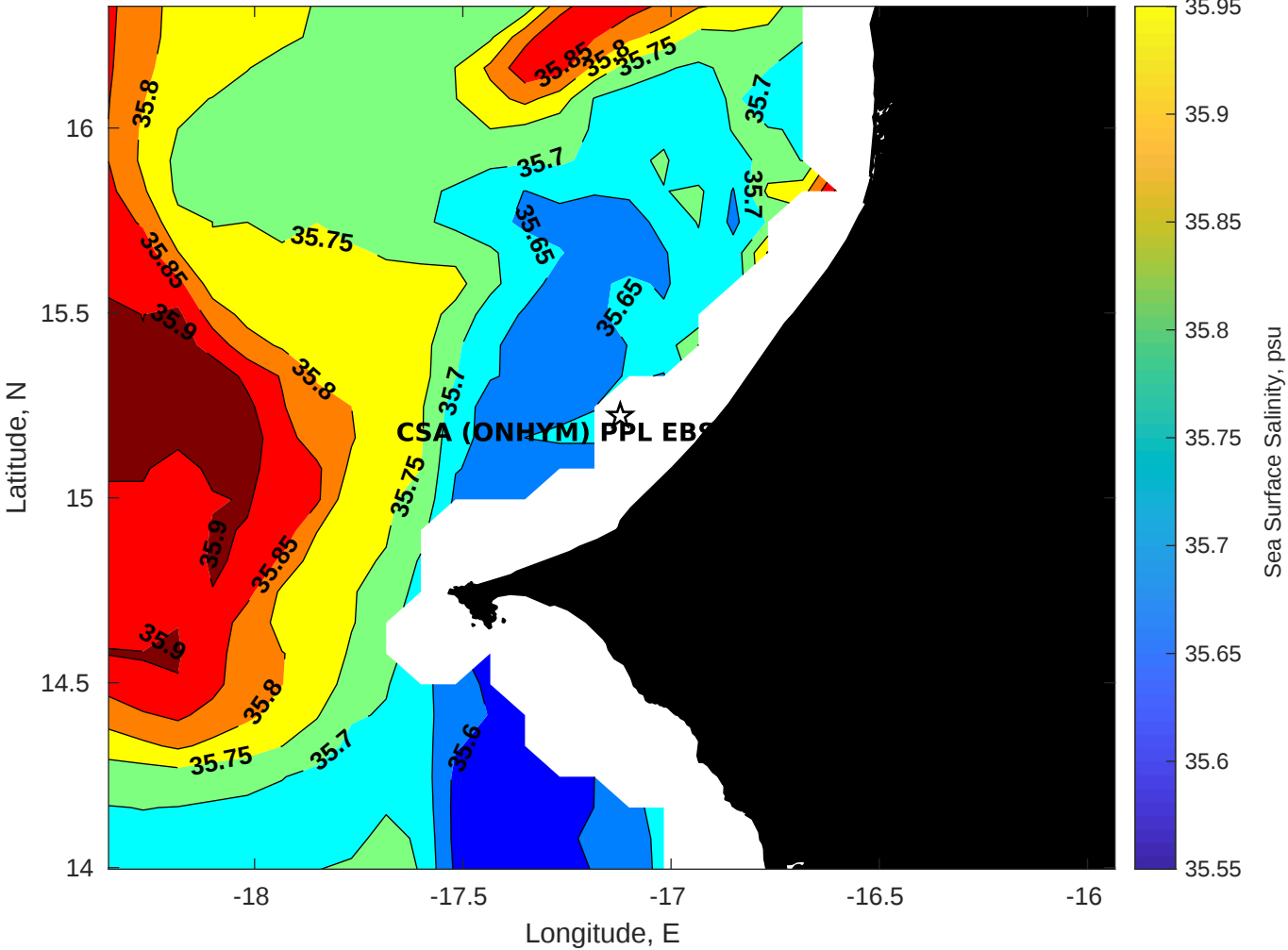
Surface Salinity for CSA (ONHYM) PPL EBS - Senegal at 07-Apr-2025 00:00:00
