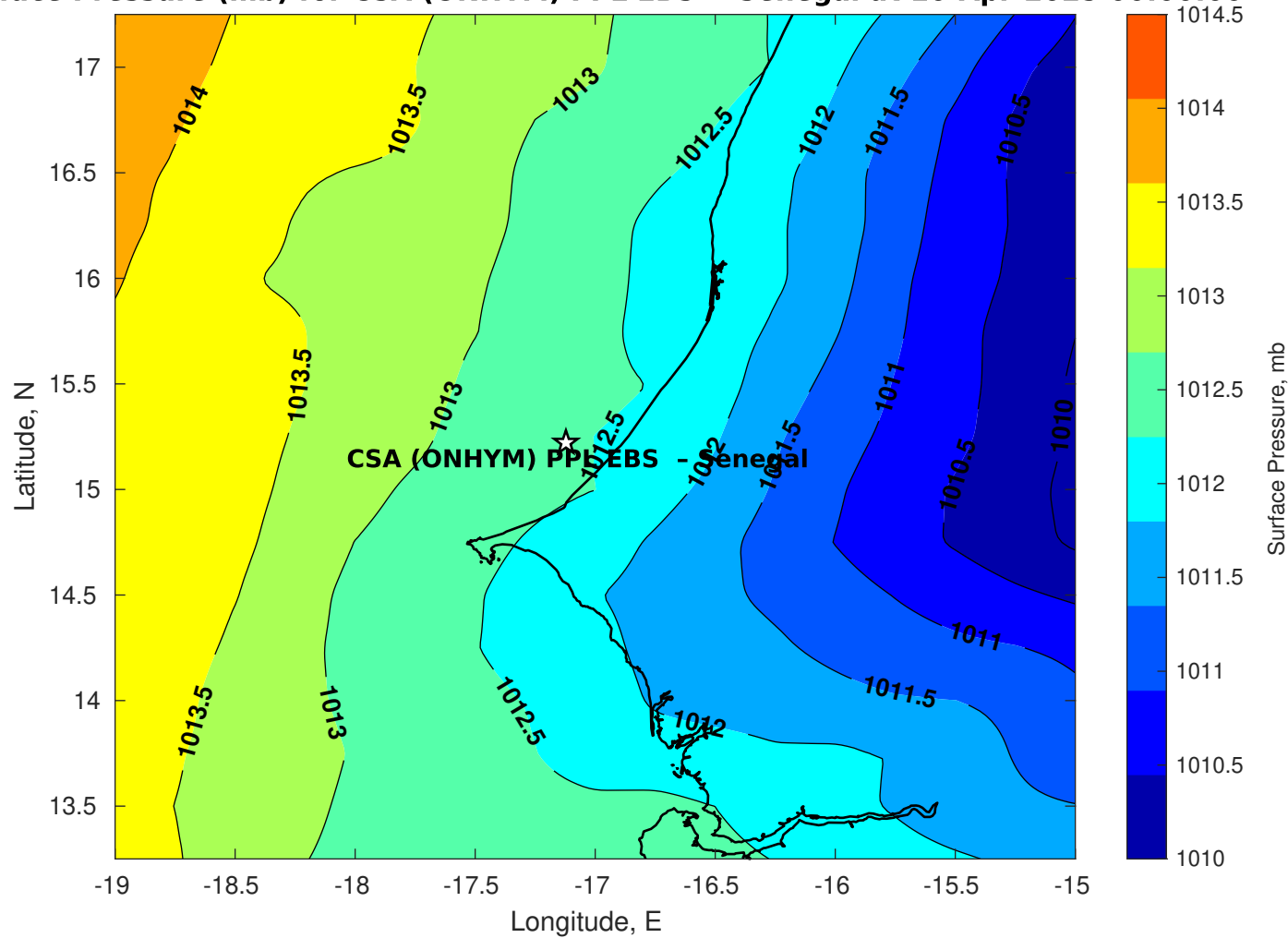
Surface Pressure (mb) for CSA (ONHYM) PPL EBS - Senegal at 10-Apr-2025 00:00:00
