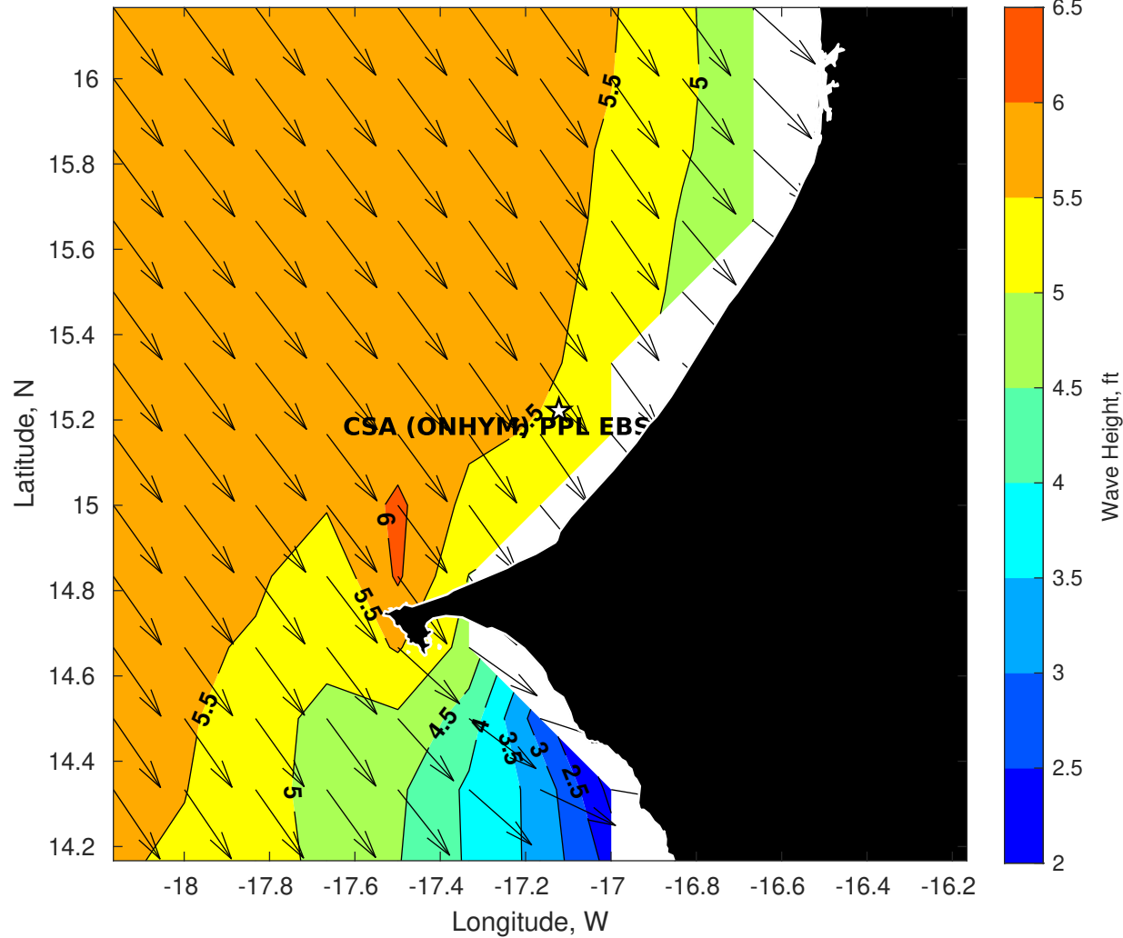
Wave Height (ft) for CSA (ONHYM) PPL EBS - Senegal at 08-Apr-2025 09:00:00
