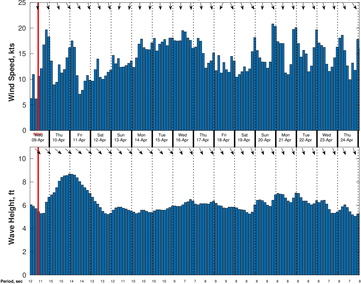
Wind & Wave Forecast for CSA (ONHYM) PPL EBS - Senegal from 08-Apr-2025 01:00:00 to 24-Apr-2025 01:00:00
