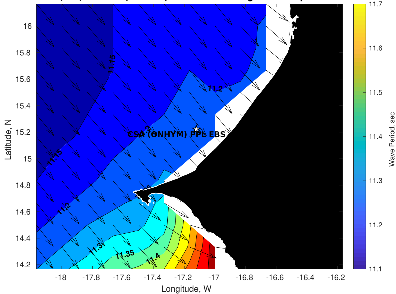
Wave Period (sec) for CSA (ONHYM) PPL EBS - Senegal at 08-Apr-2025 09:00:00
