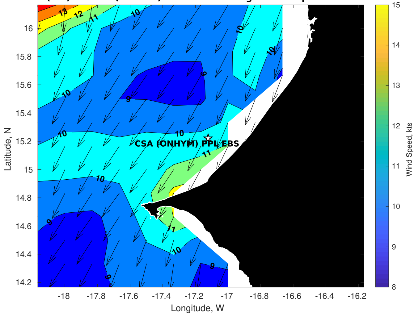
Winds (kts) for CSA (ONHYM) PPL EBS - Senegal at 08-Apr-2025 09:00:00
