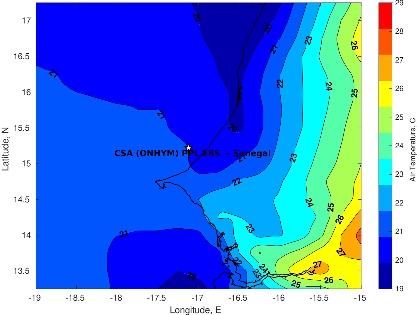
Air Temperature (C) for CSA (ONHYM) PPL EBS - Senegal at 08-Apr-2025
