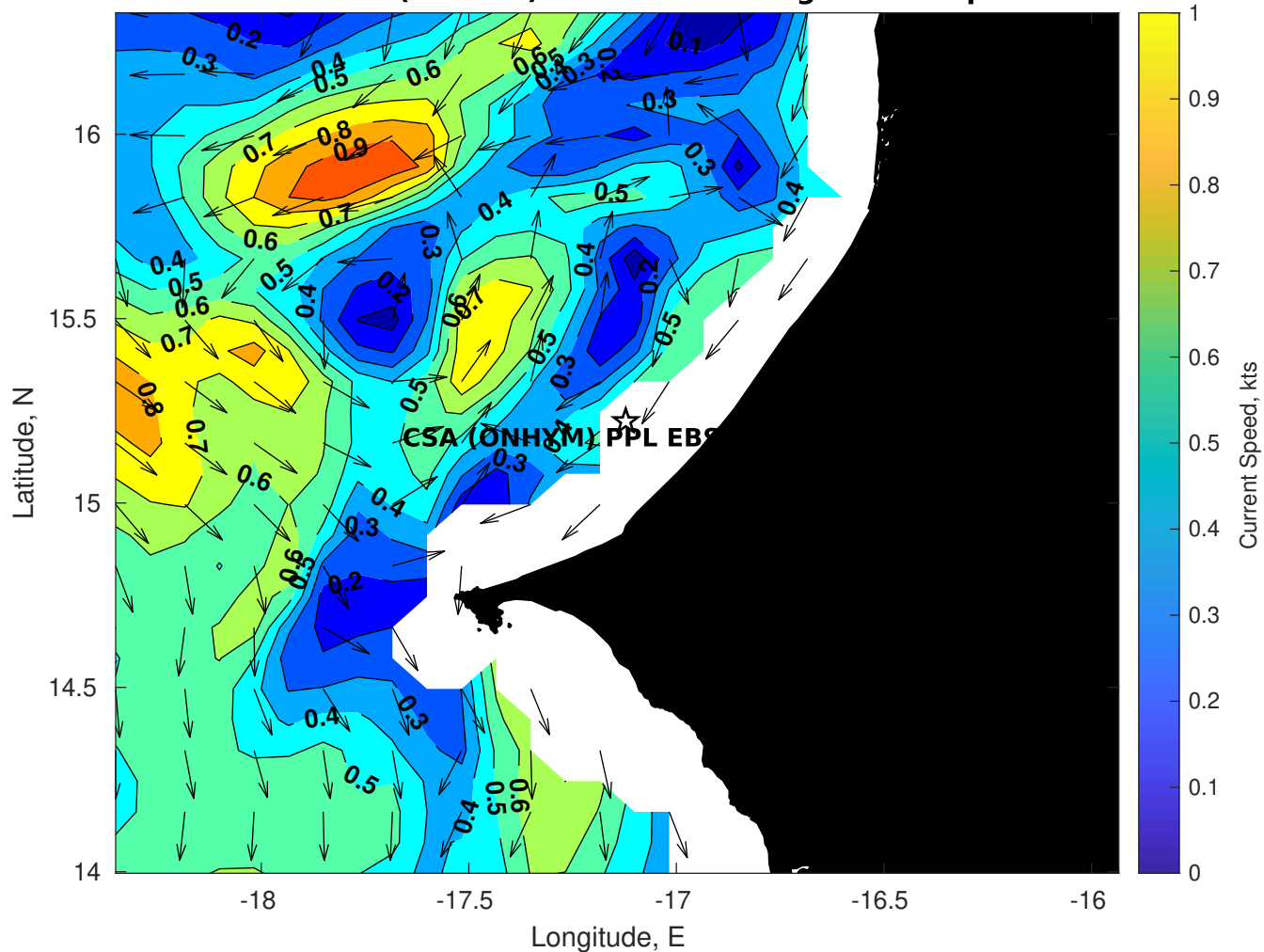
Surface Currents for CSA (ONHYM) PPL EBS - Senegal at 07-Apr-2025 00:00:00
