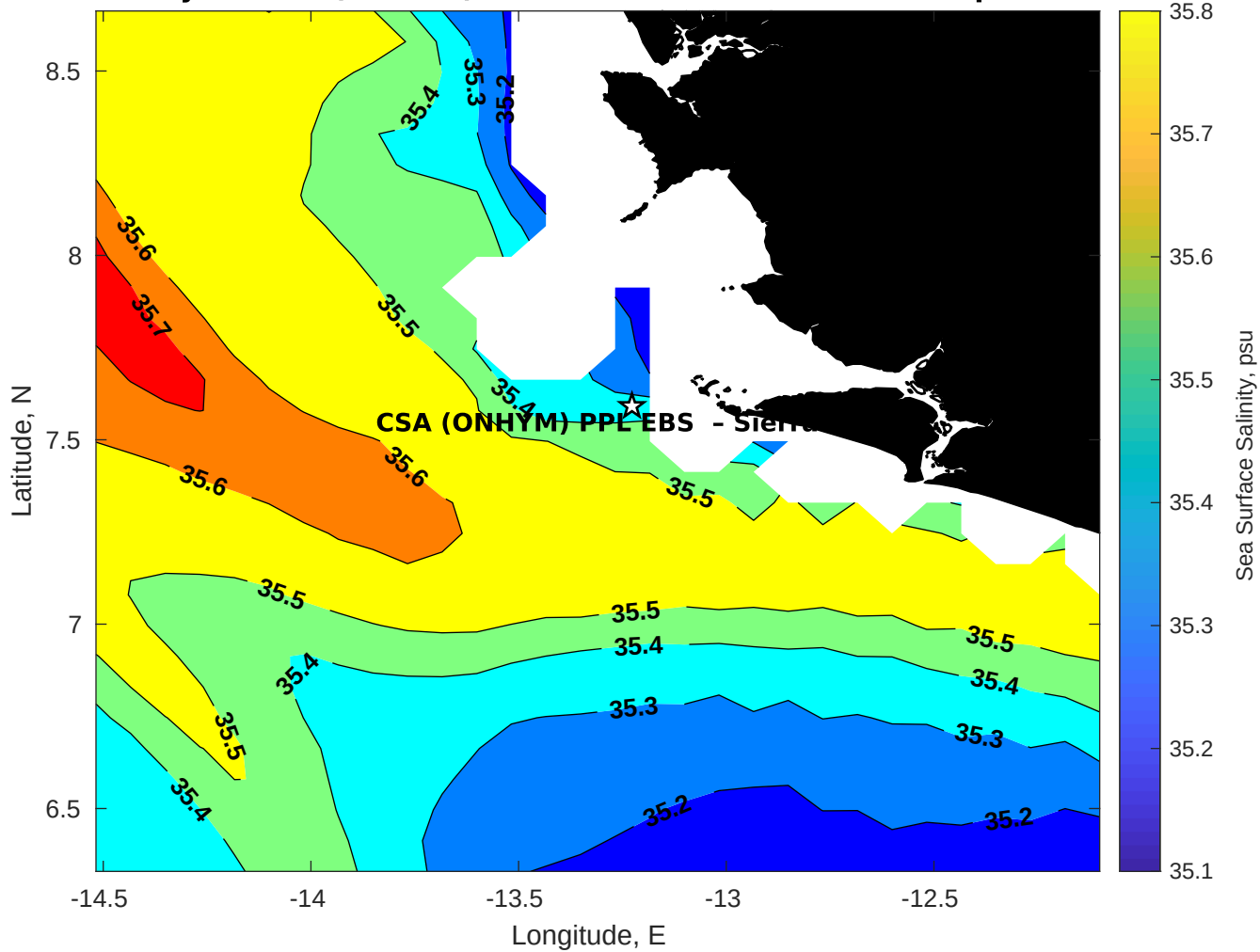
Surface Salinity for CSA (ONHYM) PPL EBS - Sierra Leone at 07-Apr-2025 00:00:00
