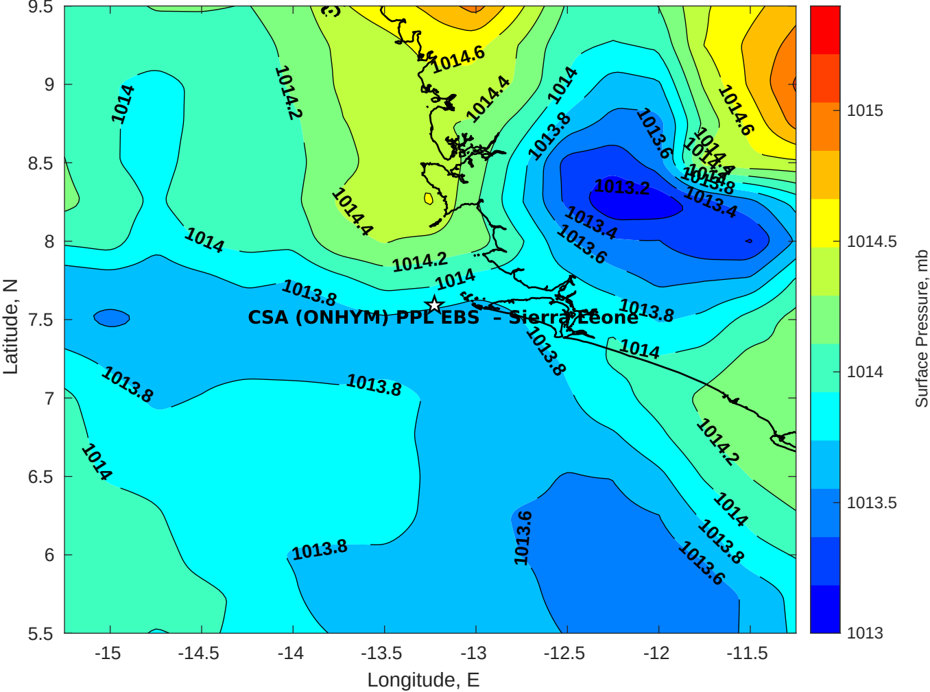
Surface Pressure (mb) for CSA (ONHYM) PPL EBS - Sierra Leone at 09-Apr-2025 00:00:00
