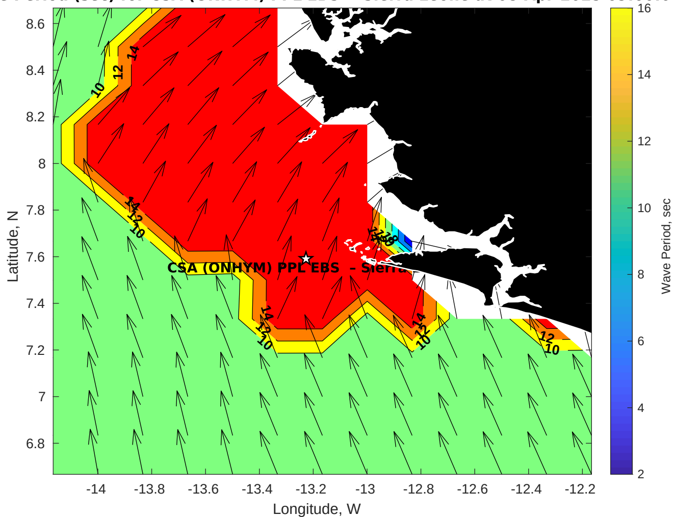
Wave Period (sec) for CSA (ONHYM) PPL EBS - Sierra Leone at 08-Apr-2025 09:00:00
