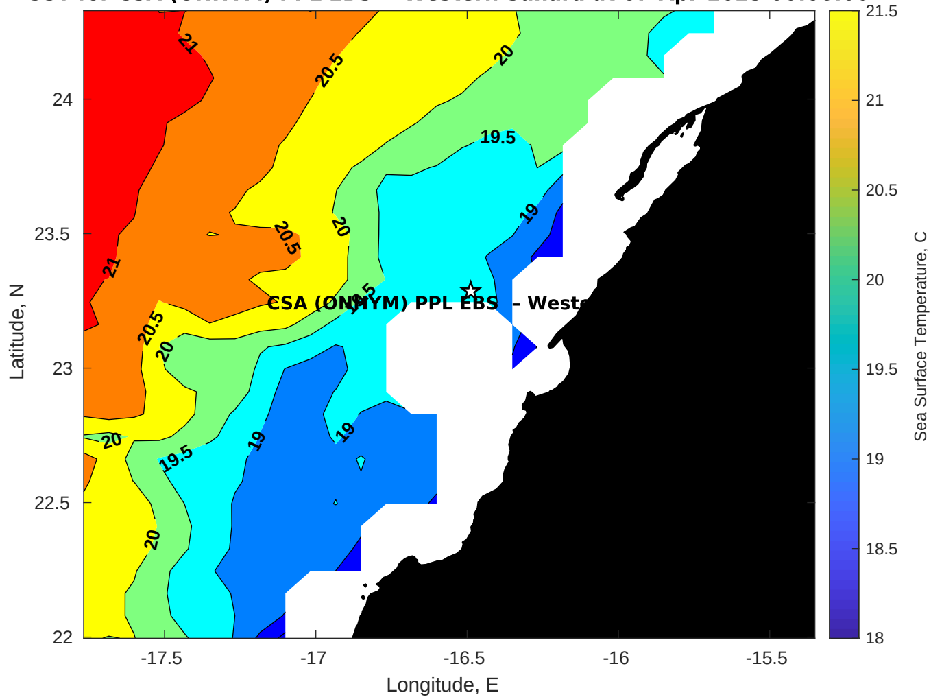
SST for CSA (ONHYM) PPL EBS - Western Sahara at 07-Apr-2025 00:00:00
