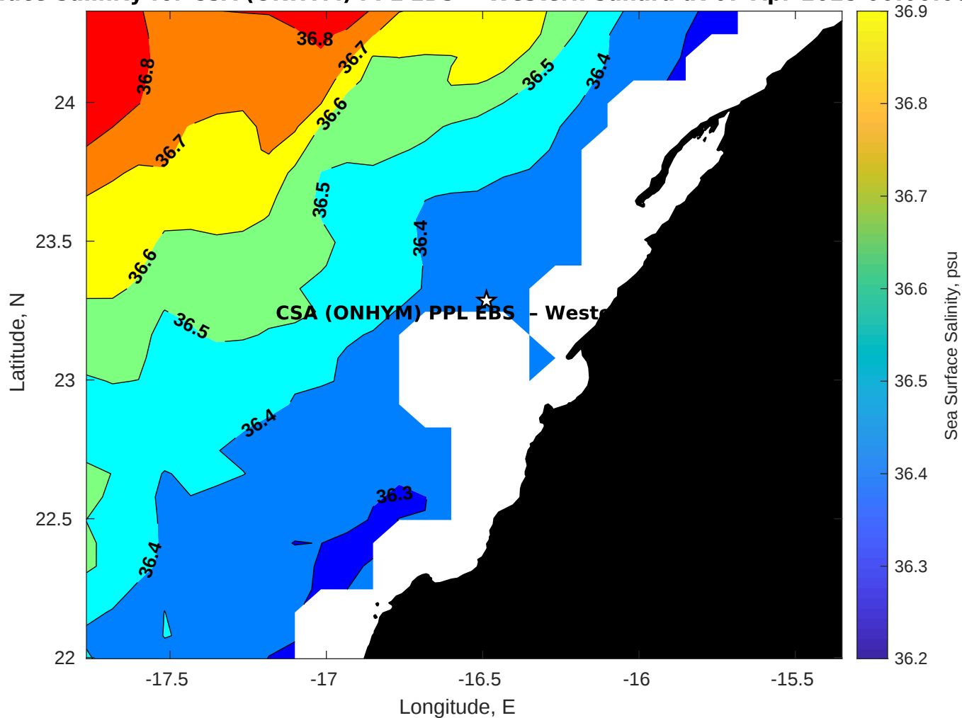
Surface Salinity for CSA (ONHYM) PPL EBS - Western Sahara at 07-Apr-2025 00:00:00
