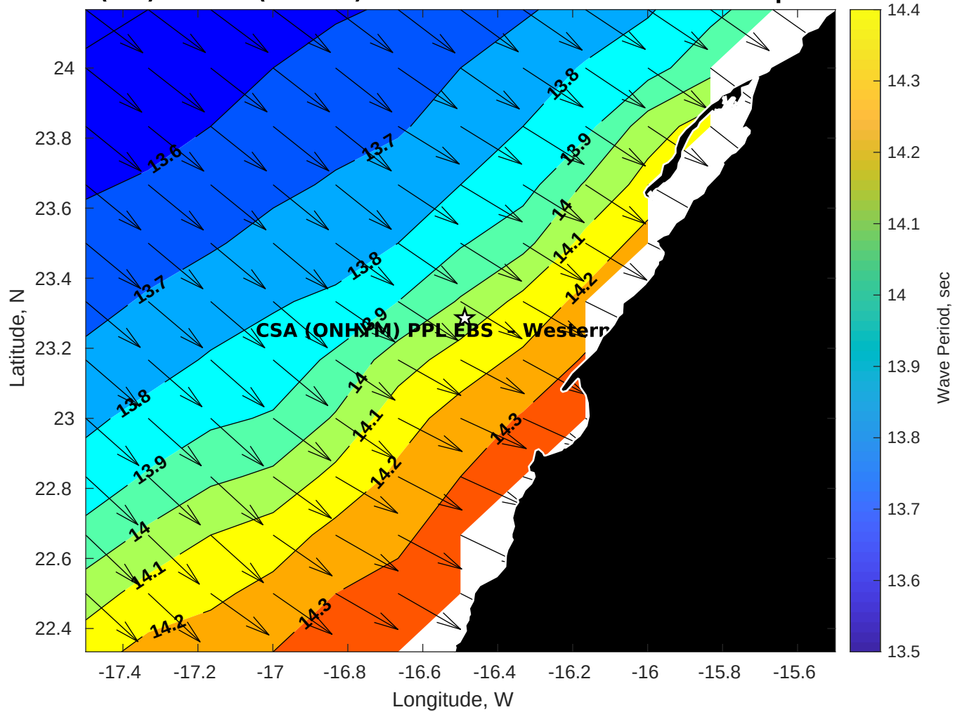
Wave Period (sec) for CSA (ONHYM) PPL EBS - Western Sahara at 08-Apr-2025 09:00:00
