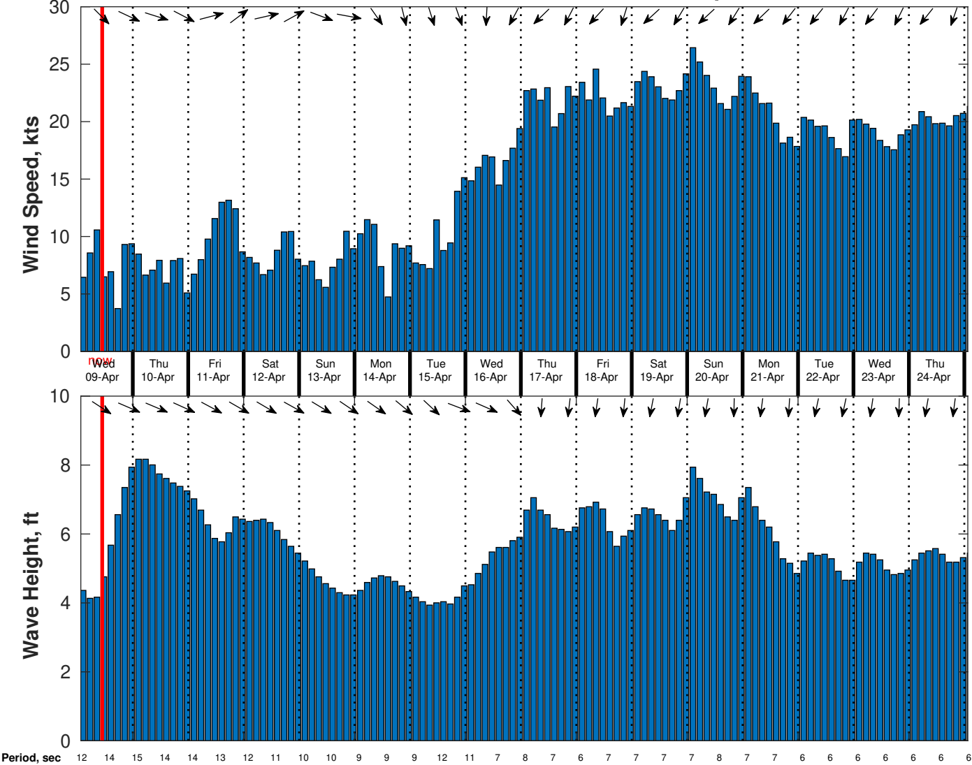
Wind & Wave Forecast for CSA (ONHYM) PPL EBS - Western Sahara from 08-Apr-2025 01:00:00 to 24-Apr-2025 01:00:00
