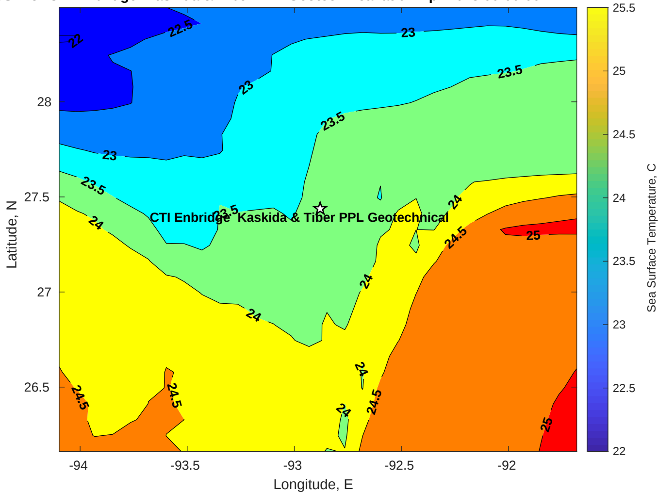
SST for CTI Enbridge Kaskida & Tiber PPL Geotechnical at 07-Apr-2025 00:00:00
