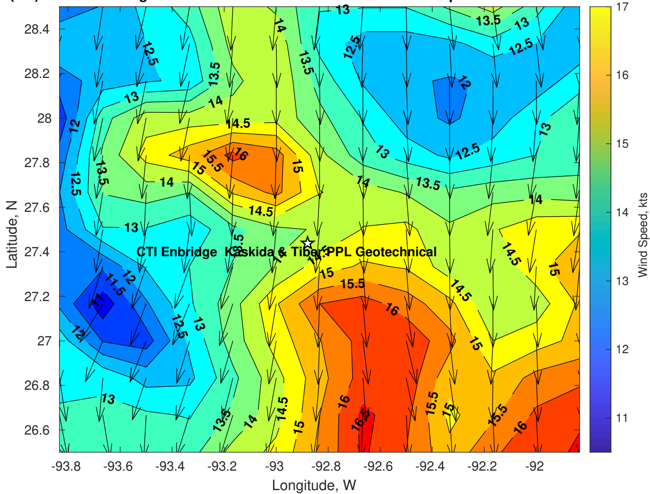
Winds (kts) for CTI Enbridge Kaskida & Tiber PPL Geotechnical at 08-Apr-2025 09:00:00
