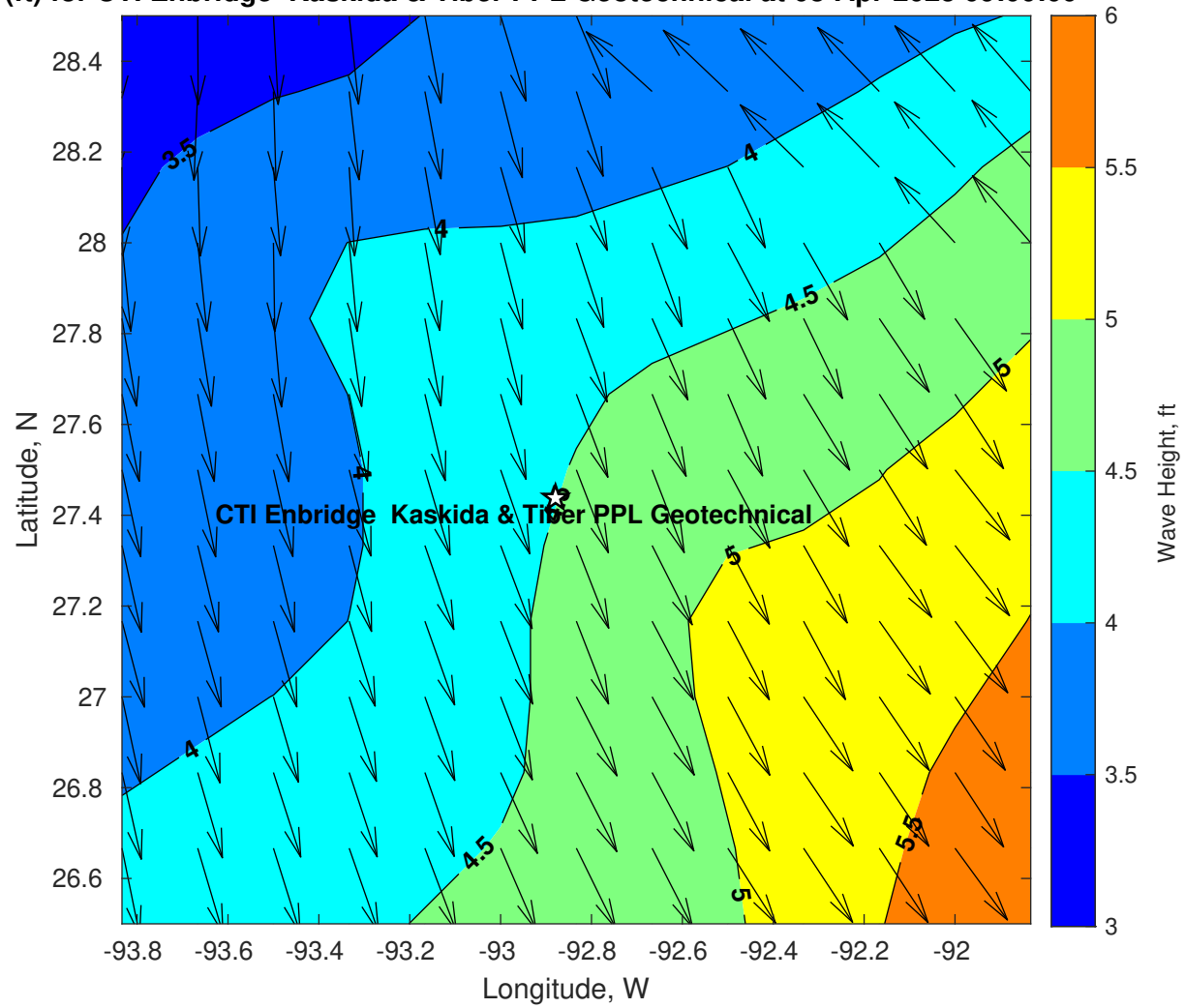
Wave Height (ft) for CTI Enbridge Kaskida & Tiber PPL Geotechnical at 08-Apr-2025 09:00:00
