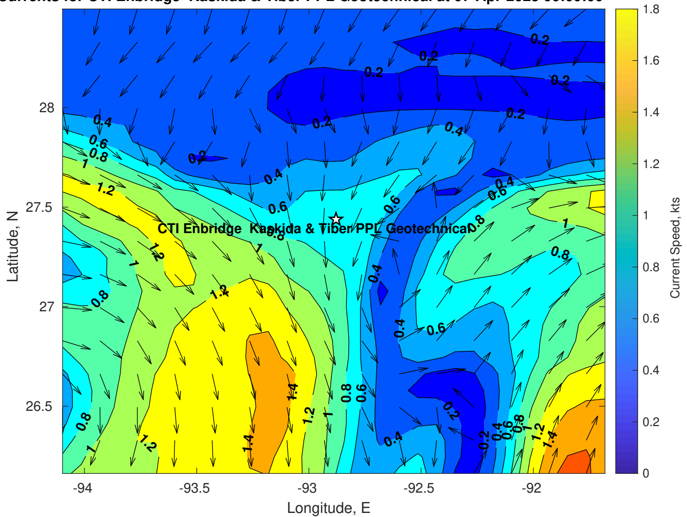
Surface Currents for CTI Enbridge Kaskida & Tiber PPL Geotechnical at 07-Apr-2025 00:00:00
