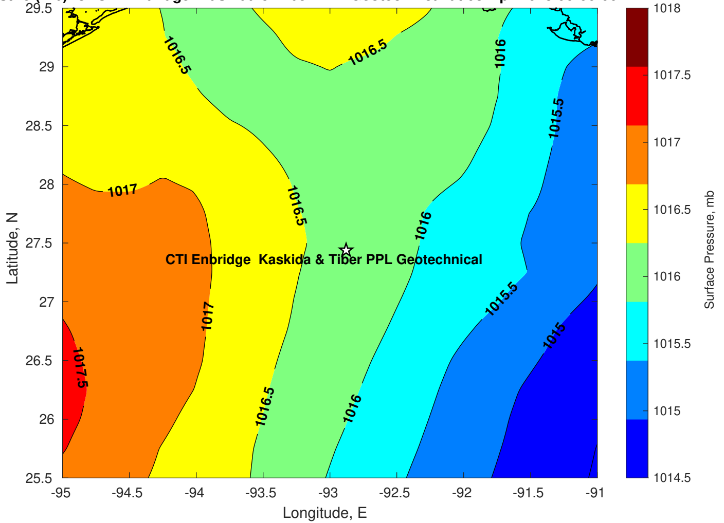
Surface Pressure (mb) for CTI Enbridge Kaskida & Tiber PPL Geotechnical at 08-Apr-2025 00:00:00
