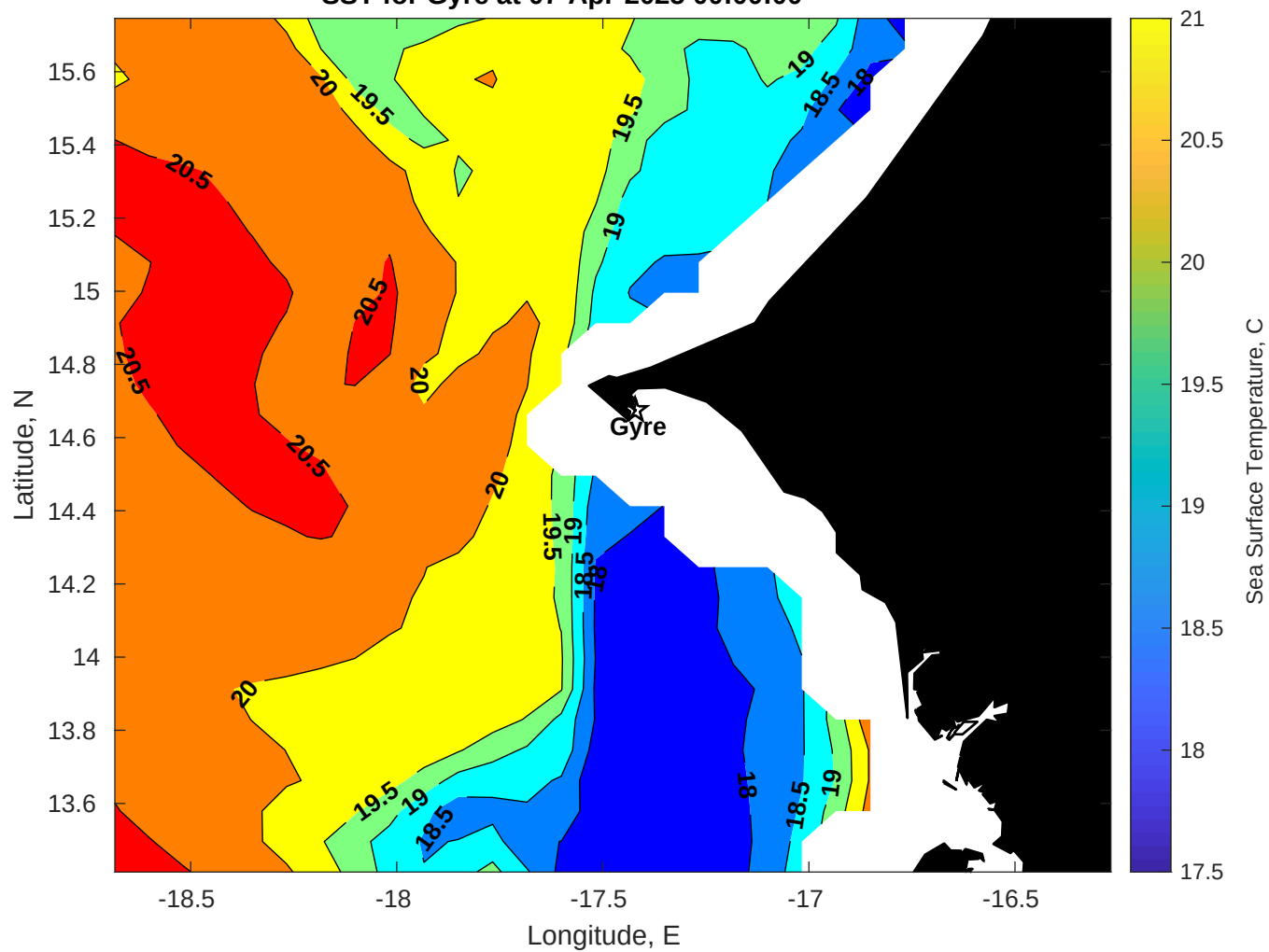
SST for Gyre at 07-Apr-2025 00:00:00
