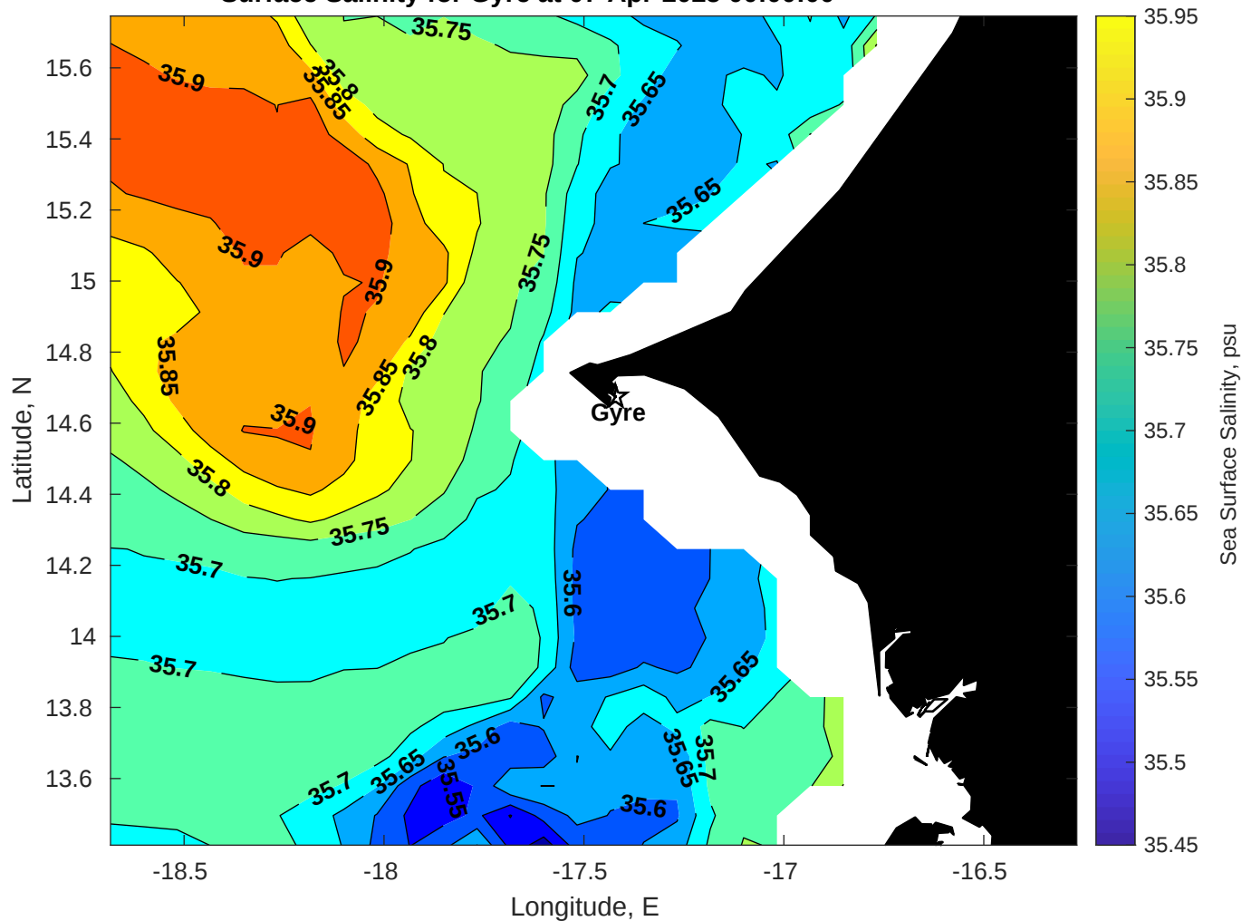
Surface Salinity for Gyre at 07-Apr-2025 00:00:00
