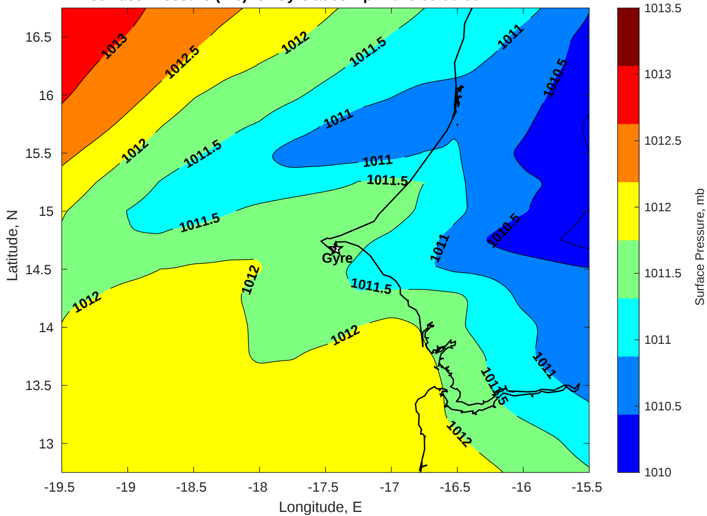
Surface Pressure (mb) for Gyre at 08-Apr-2025 00:00:00
