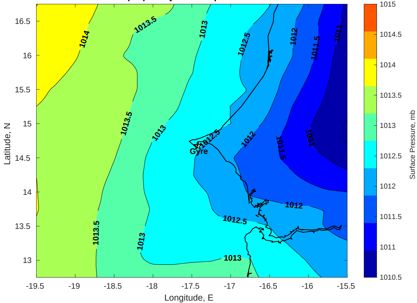
Surface Pressure (mb) for Gyre at 10-Apr-2025 00:00:00
