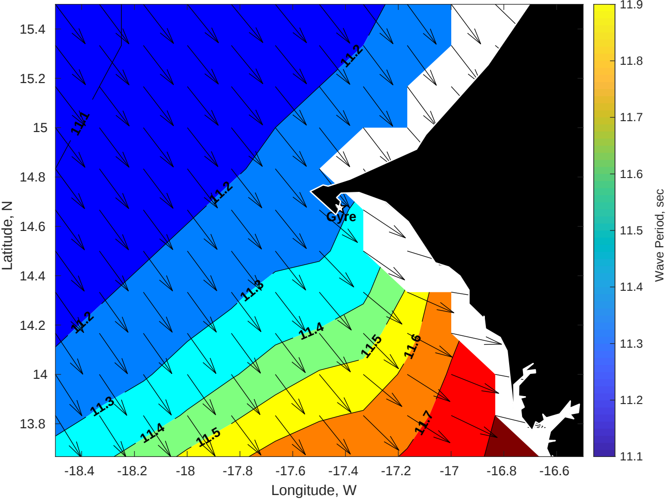
Wave Period (sec) for Gyre at 08-Apr-2025 09:00:00
