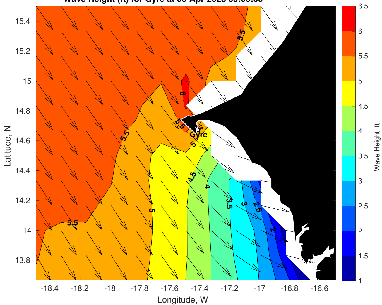
Wave Height (ft) for Gyre at 08-Apr-2025 09:00:00
