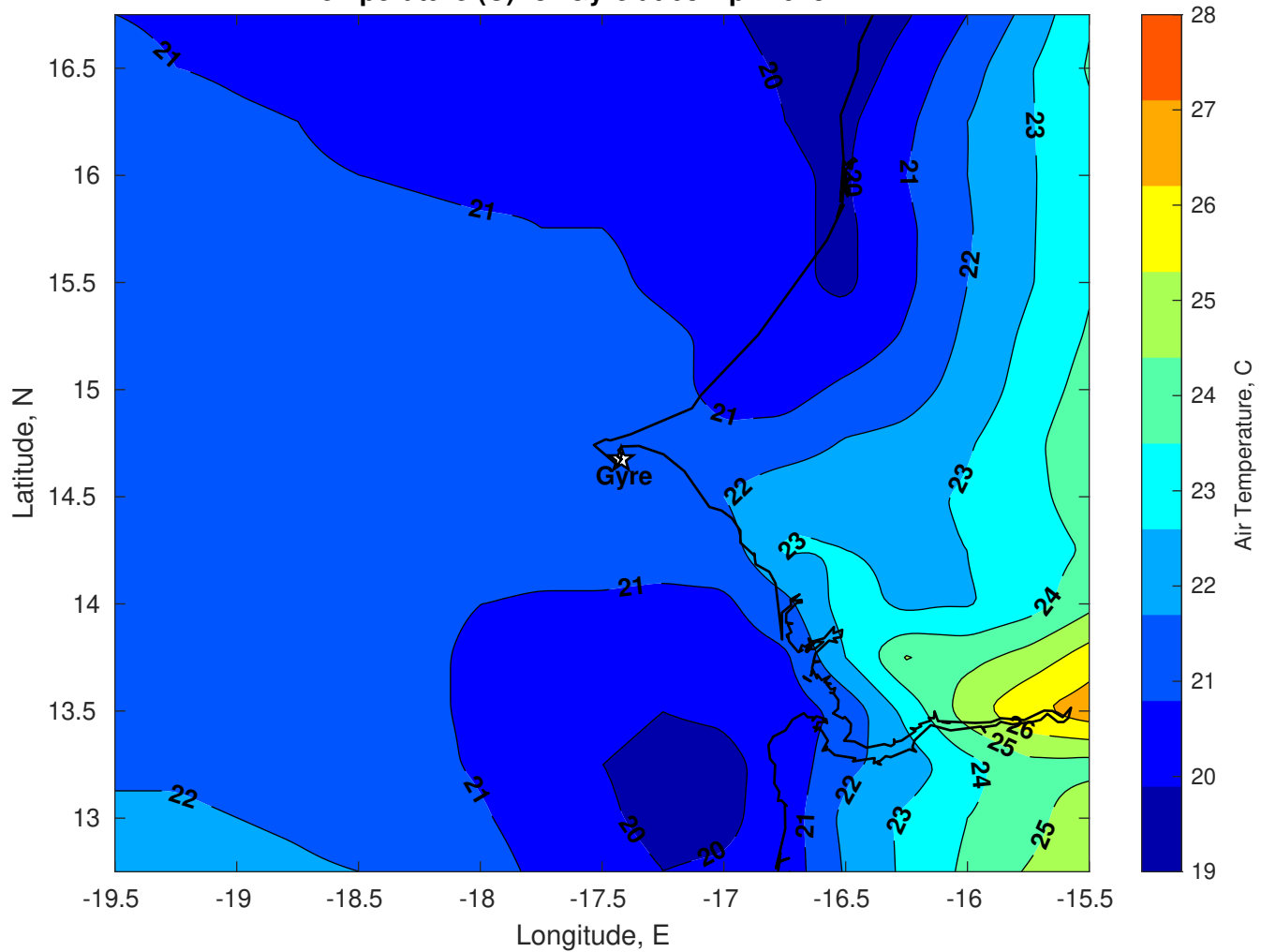
Air Temperature (C) for Gyre at 08-Apr-2025
