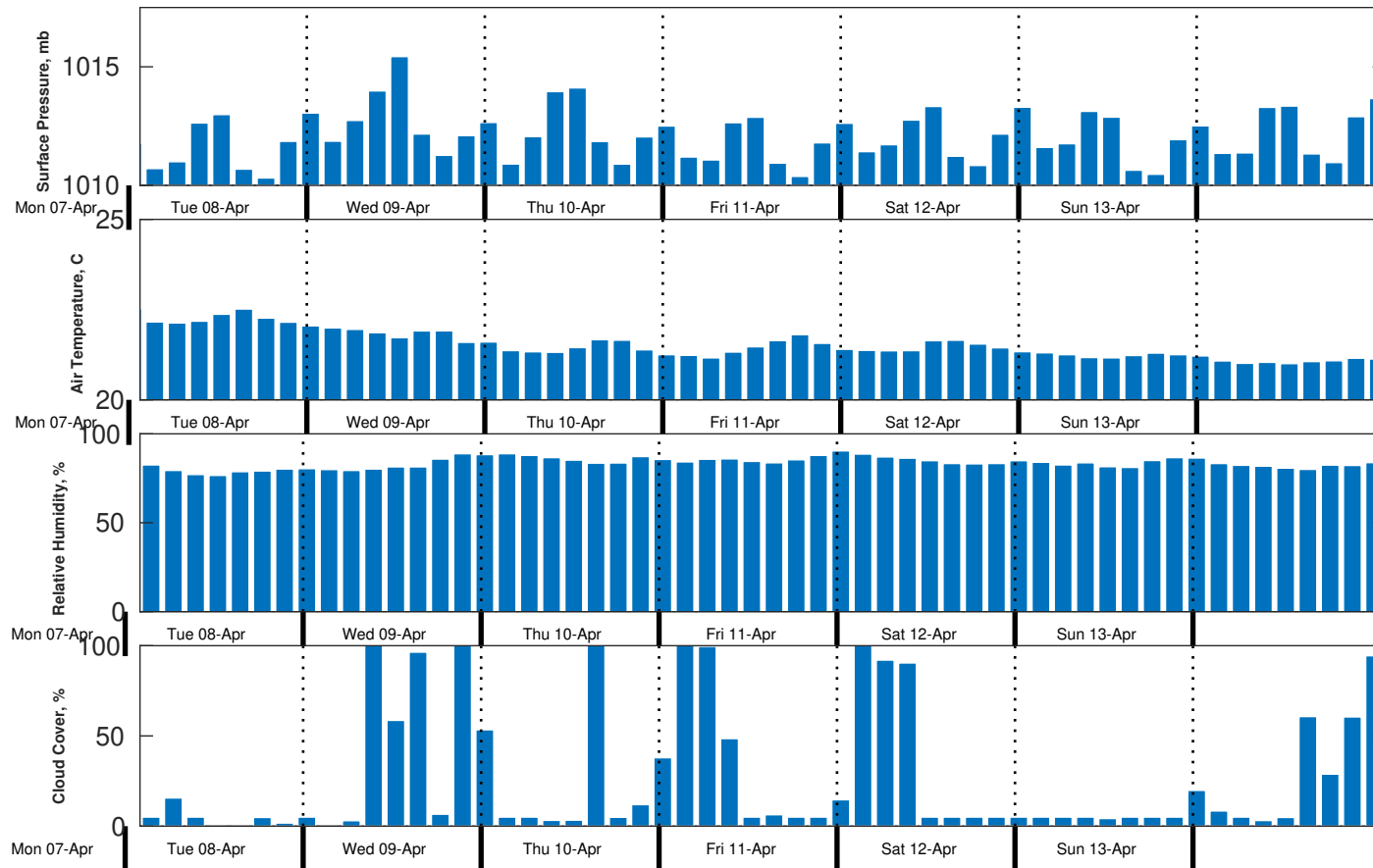
Met Forecast for Gyre from 07-Apr-2025 23:00:00 to 14-Apr-2025 23:00:00
