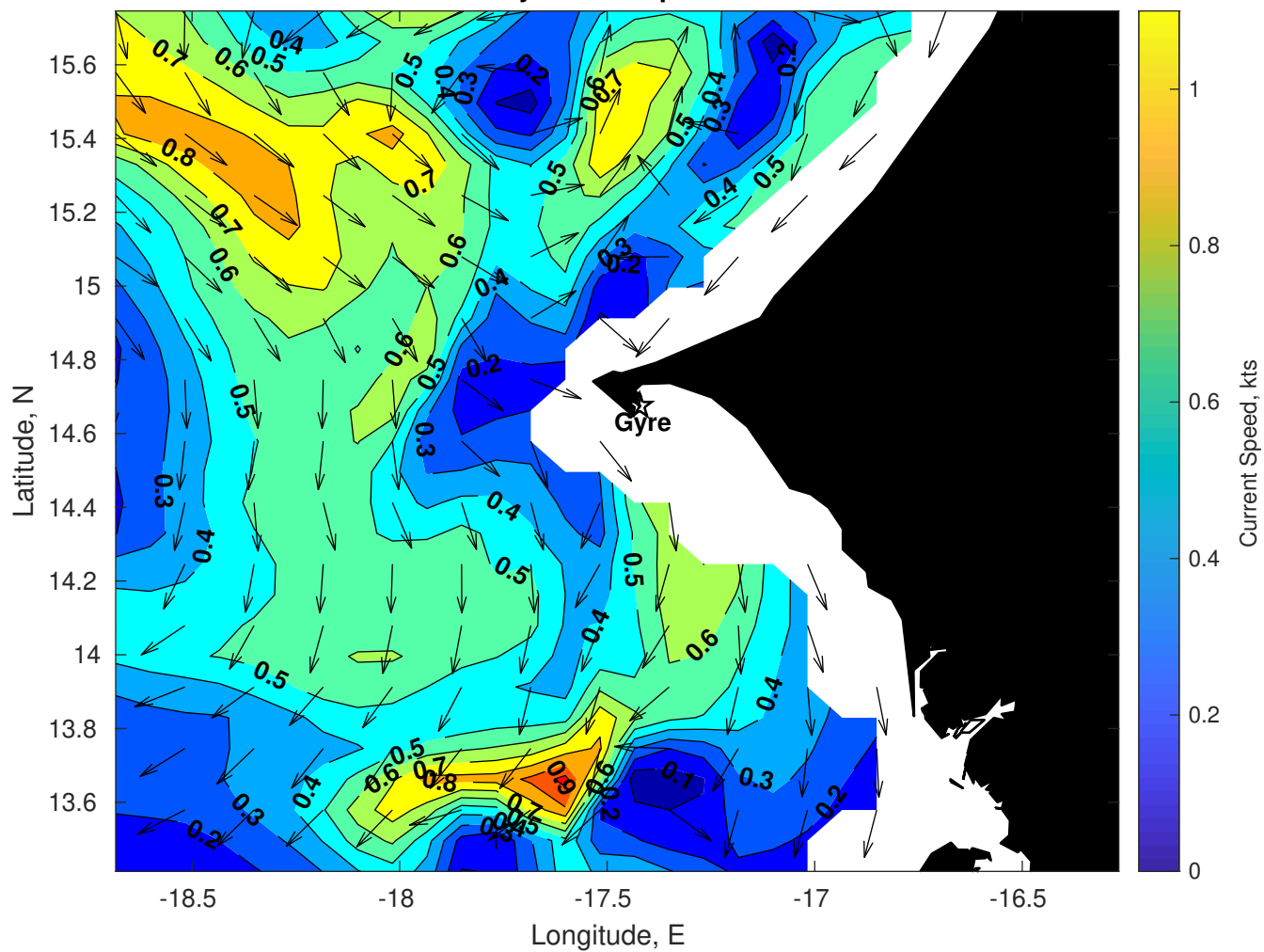
Surface Currents for Gyre at 07-Apr-2025 00:00:00
