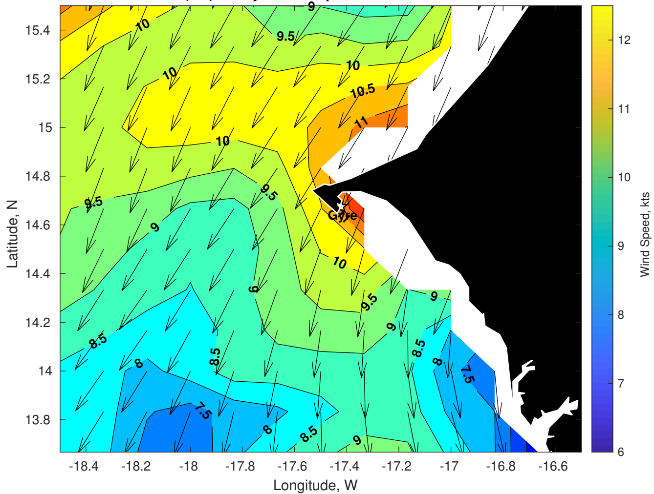
Winds (kts) for Gyre at 08-Apr-2025 09:00:00
