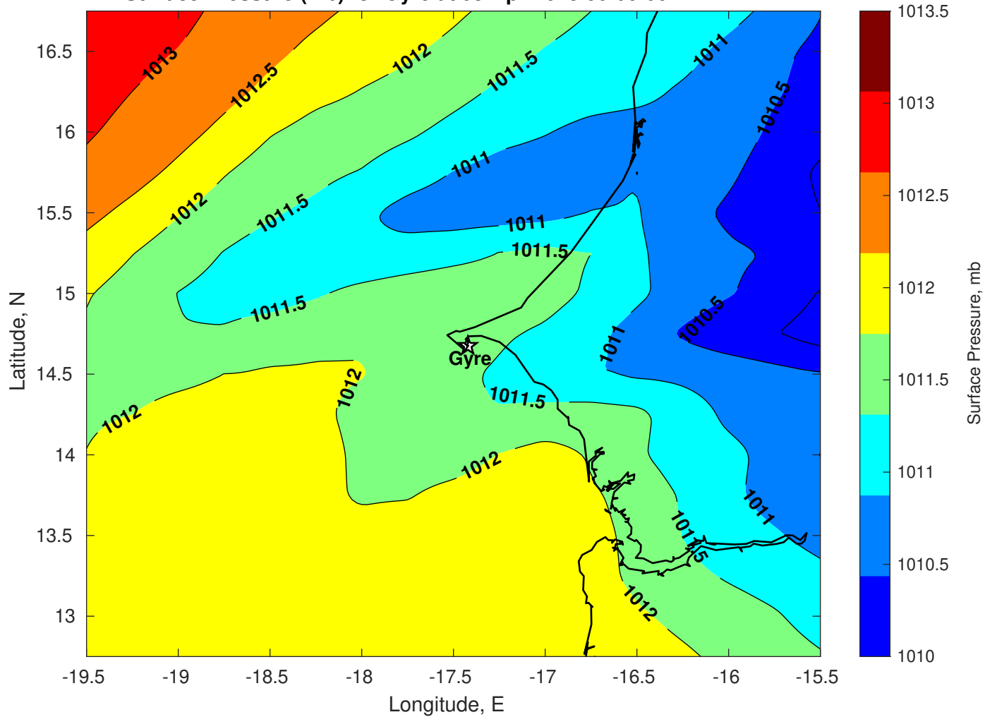
Surface Pressure (mb) for Gyre at 08-Apr-2025 00:00:00
