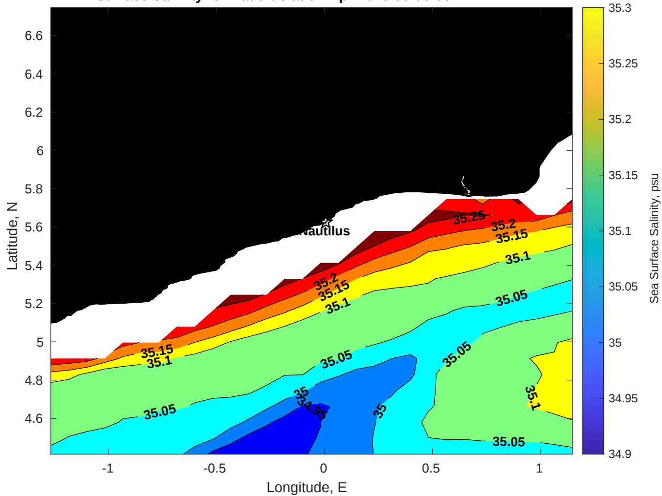
Surface Salinity for Nautilus at 07-Apr-2025 00:00:00
