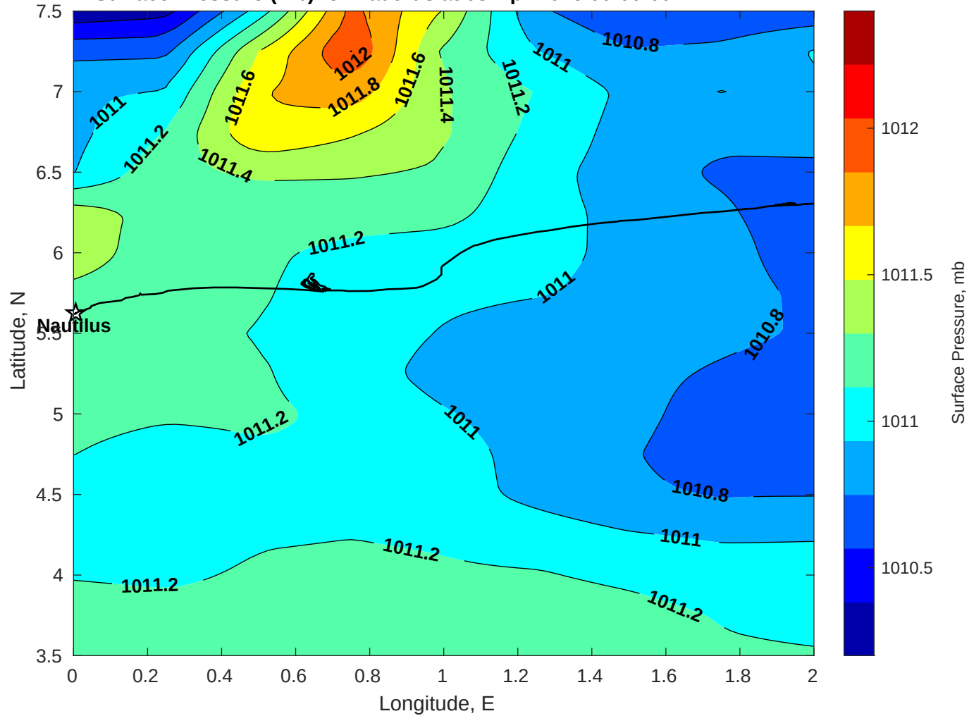
Surface Pressure (mb) for Nautilus at 08-Apr-2025 00:00:00
