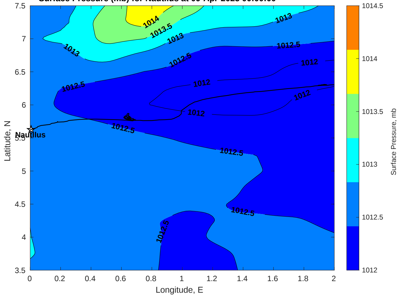
Surface Pressure (mb) for Nautilus at 09-Apr-2025 00:00:00
