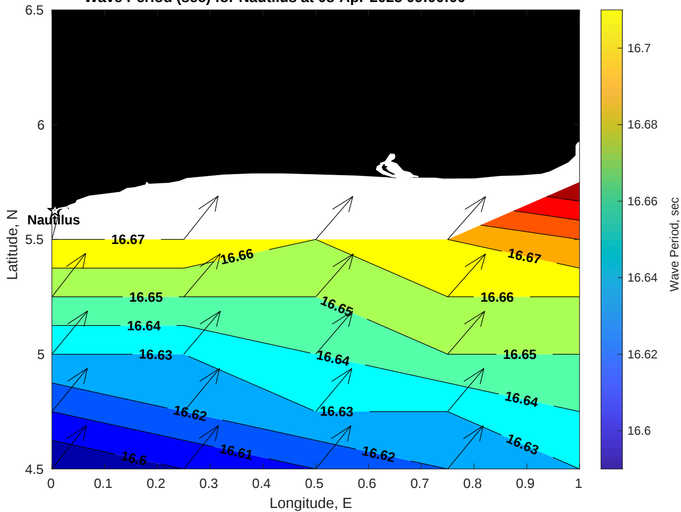
Wave Period (sec) for Nautilus at 08-Apr-2025 09:00:00
